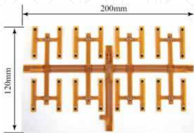
Fig. 8. Tactile sensor sheet (Ohmura 2007)
