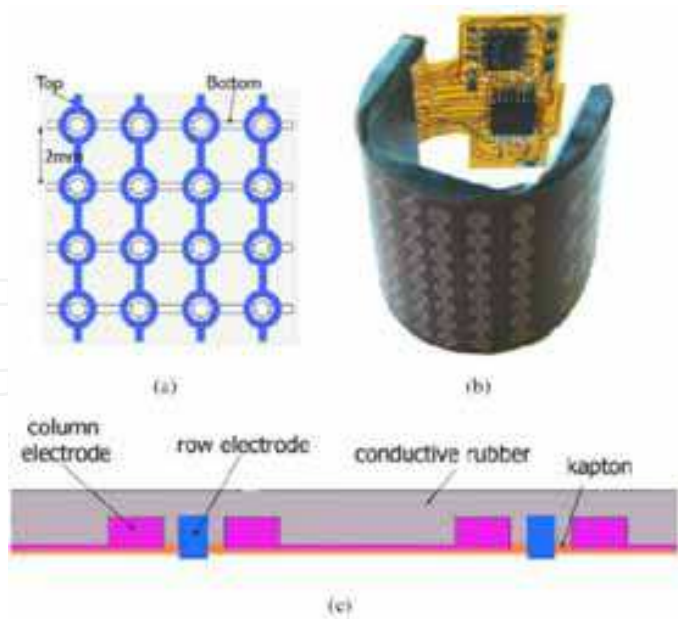
Fig. 19. The electrodes of the tactile sensor are etched on a double layer flex-PCB, and are connected in a matrix configuration (fig. a).The flex circuit conforms to the cylindrical phalange rigid cover (fig. b - resistive rubber not shown here). Fig. c: section view of the tactile sensor. Row electrodes are encircled by column electrodes.
