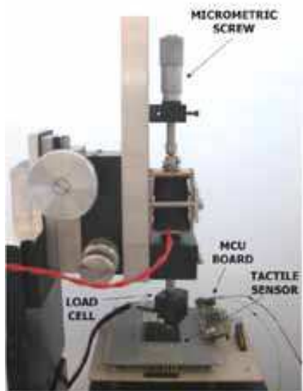
Fig. 22. Test rig for sensor calibration and tests.
