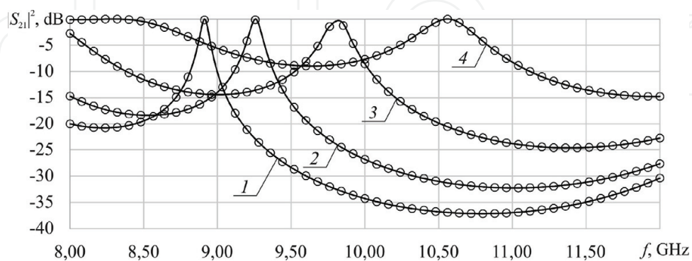
Figure 6. Amplitude-frequency characteristics of the transmission coefficients of a photonic crystal calculated using the values of the effective permittivity \varepsilon_{ef} found from the inverse problem solution, of ceramics layers with different fraction of air inclusions with the disturbed sixth layer of 6.0 mm, \varepsilon_{ef} , rel. units: 1–9.6 ( x_1 = 0\% ), 2–8.44 ( x_1 = 8.5\% ), 3–6.78 ( x_1 = 23.0\% ), 4–4.82 ( x_1 = 43.0\% ).
