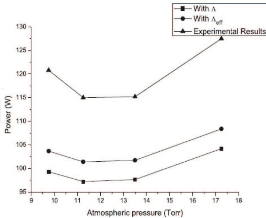
Figure 4. Experimental and analytical results using \Lambda and \Lambda_{eff} for a Ku band filter operating at 12.5 GHz.
