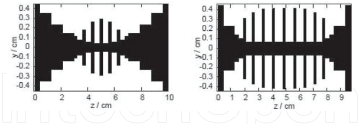
Figure 6. Transversal configuration of waveguide filters. (a) Operating at 12.2 GHz. (b) Operating at 12.5 GHz [4].
