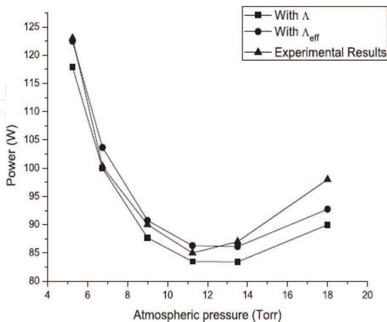
Figure 5. Experimental and analytical results using \Lambda and \Lambda_{eff} for a Ku band filter operating at 12.2 GHz.
