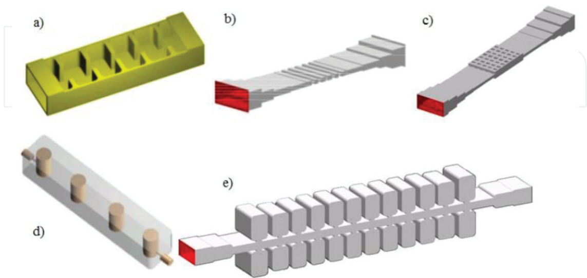
Figure 1. (a) Coupled iris filter, (b) corrugated waveguide filter, (c) waffle iron filter, (d) posts filter, and (e) guarded waveguide filter.
