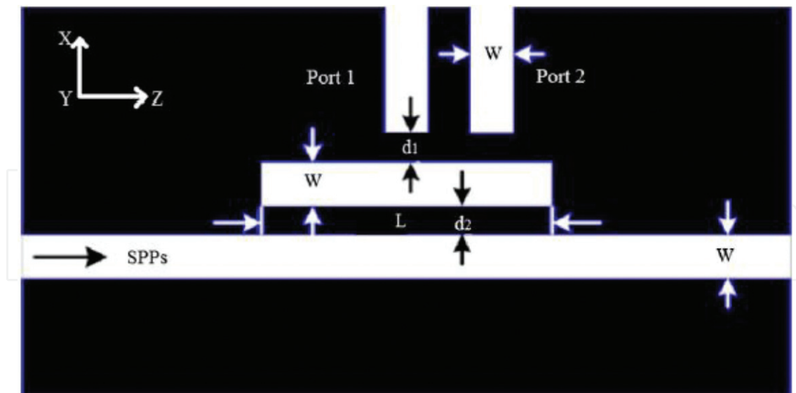
Figure 11. Two-channel plasmonic waveguide filter structure.
