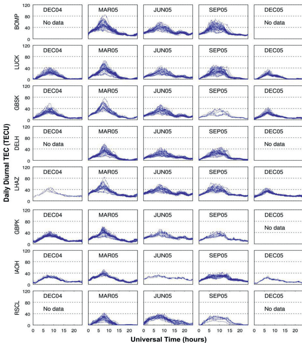
Figure 5. Daily diurnal GPS TEC during solar cycle 23 (2004–2005) for cGPS stations above 17^\circ N geomagnetic latitude.
