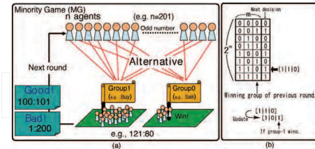
Fig. 1. Rule of MG and detail of strategy table.
