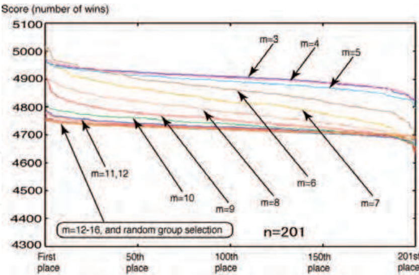
Fig. 3. Rankings of agents for each m after 10,000 rounds.
