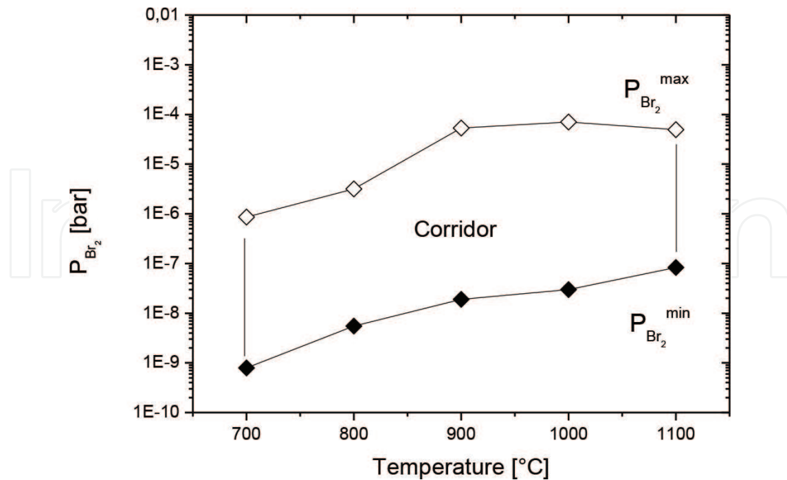
Figure A2. P_{Br_2} limits for the bromine effect.
