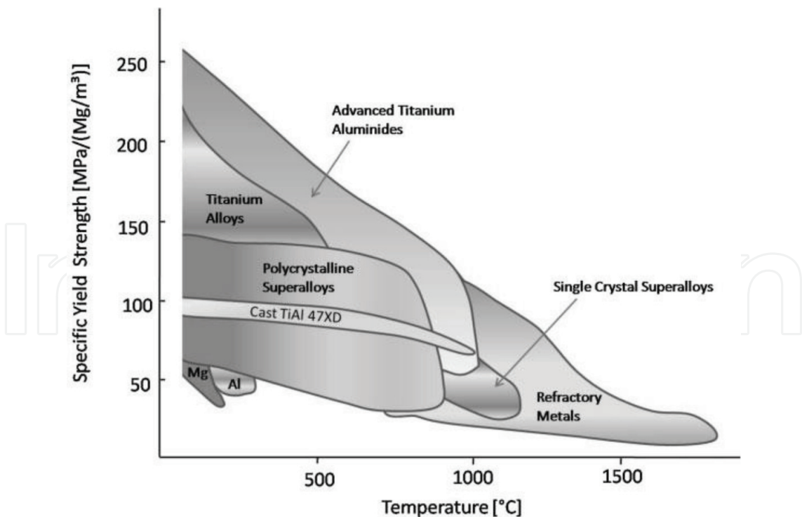
Figure 1. Comparison of the specific yield strength of engineering materials, which are used in automotive engines and in aeroengines. The figure shows that advanced titanium aluminide alloys are capable to bear higher application temperatures and loads than Ti alloys. It is evident that TiAl alloys have an advantage over Ti-based materials [1].
