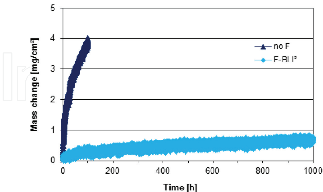
Figure 2. Thermogravimetric results of an untreated TiAl sample and a beamline fluorine-implanted TiAl sample during isothermal oxidation at 900^\circ\text{C} in air.
