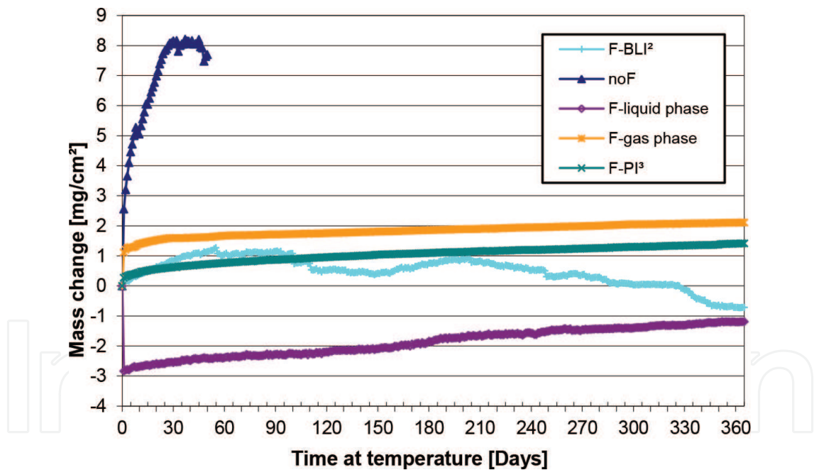
Figure 11. Mass change data of an untreated and four different F-treated specimens exposed thermocyclically at 900°C in air.
