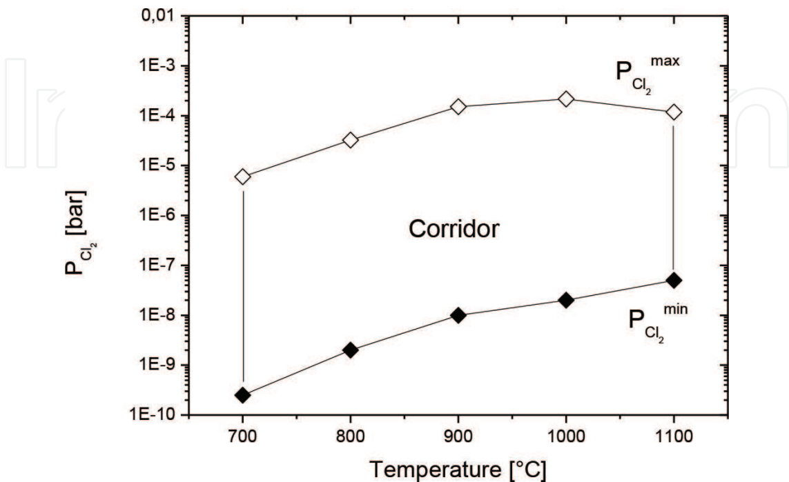
Figure A1. P_{\text{Cl}_2} limits for the chlorine effect.
