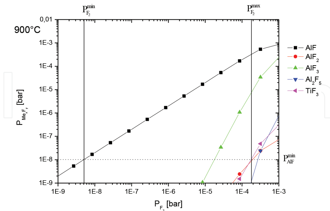
Figure 4. Calculated partial pressures of the gaseous metal fluorides versus elemental fluorine partial pressure at 900°C.
