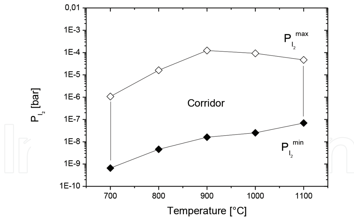
Figure A3. P_{I_2} limits for the iodine effect.
