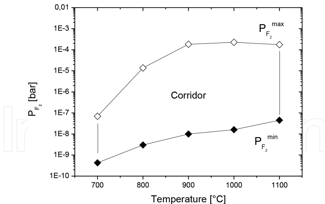
Figure 5. P_{F_2} limits of the fluorine effect.
