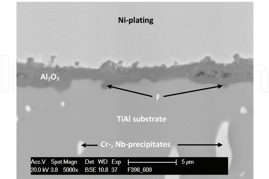
Figure 18. Corresponding SEM/BSE image of the F-PI 3 sample after thermocyclic oxidation at 900°C for 365 days in air.
