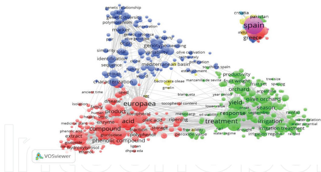
Figure 6. Co-occurrence network of terms occurred in the title and abstract of the documents on polyphenol contents and olive fruit oils between 1995 and 2017. Four clusters were identified and displayed in different colors.
