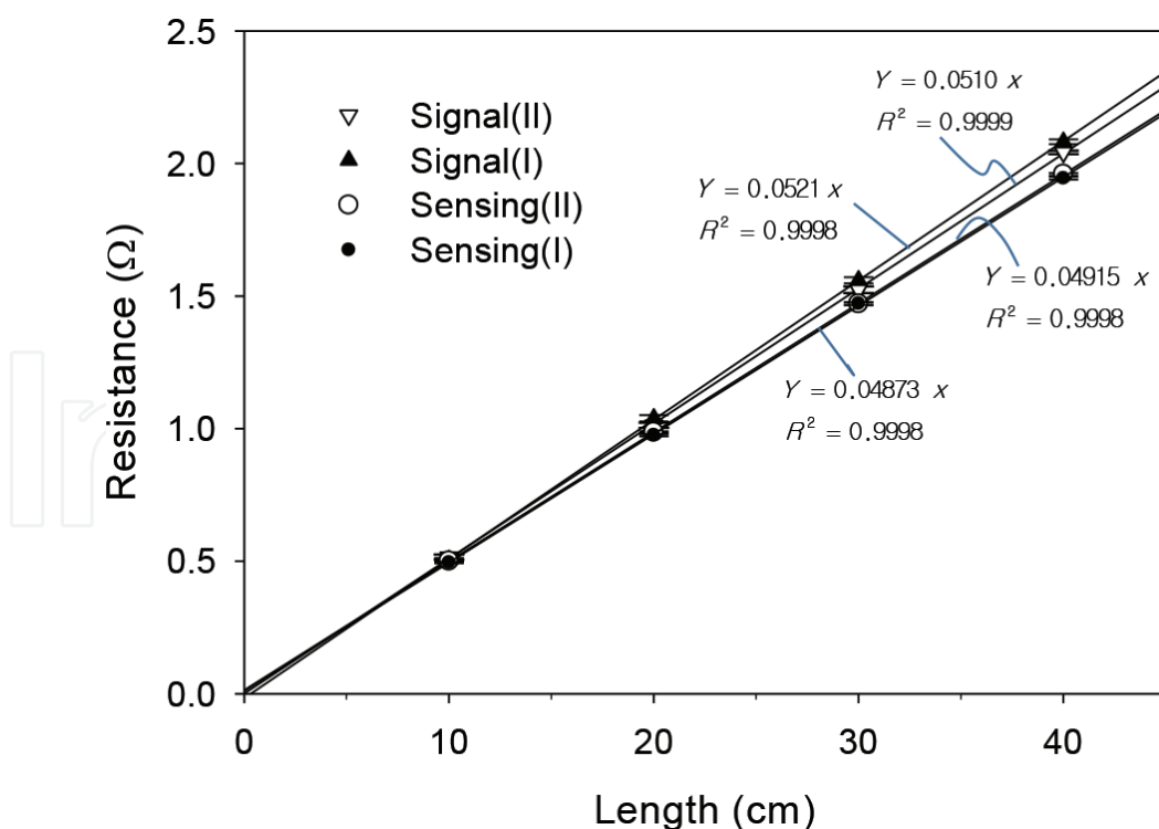
Figure 3. Electrical resistance linearity of four MCEYs as a function of the yarn length.
