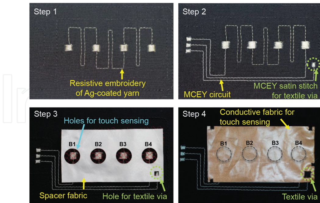
Figure 5. A one-stop production process on a standard CNC embroidery machine for fabricating the multilayer structured textile touch sensor that senses a touched position [16].
