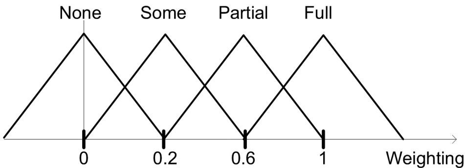
Fig. 27. Consequence membership functions for the weighting based on soft constraints. The inference engine is defined as
