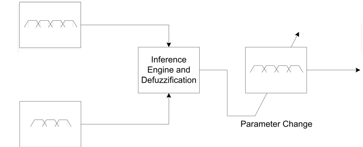
Fig. 9. A layered fuzzy system uses fuzzy logic to adjust the antecedent membership functions for another input. This reduces significantly the number of rules in the inference engines.
