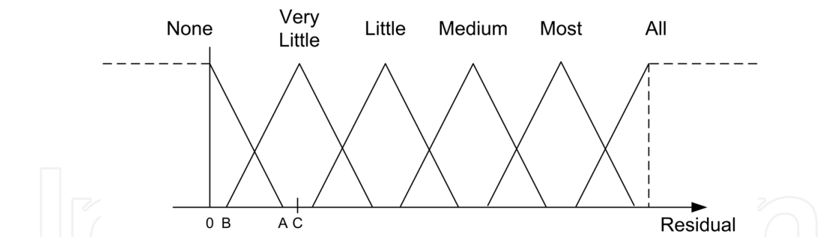
Fig. 7. Residual antecedent membership functions.
