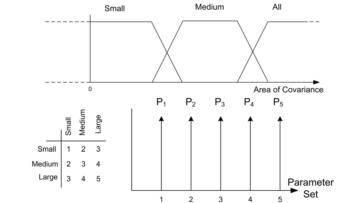
Fig. 8. Measurement and track covariances are used to determine a weighted parameter set through a fuzzy inference engine.
