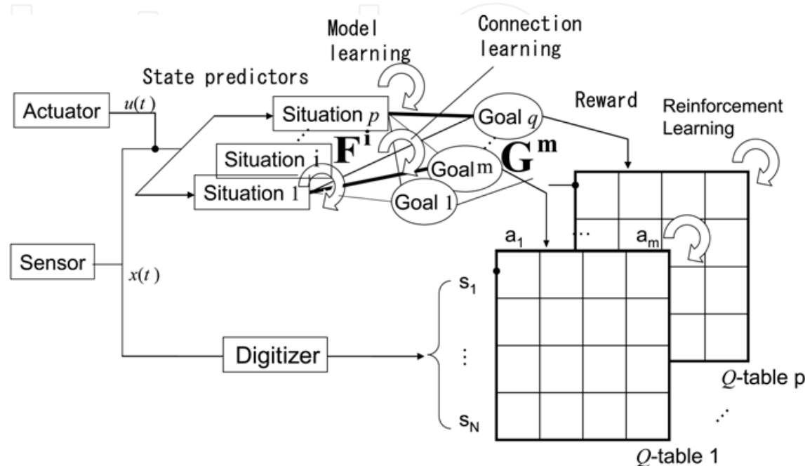
Fig. 5. Situation-Sensitive Reinforcement Learning architecture
