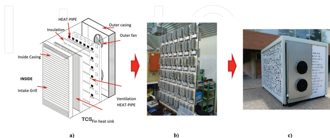
Figure 1. Schematic diagram of THU v1.1: (a) parts of the prototype, (b) heating system (heat pipes with Peltier cells) and (c) external view showing the electrical connection (down) and the ventilation grills (sideways).
