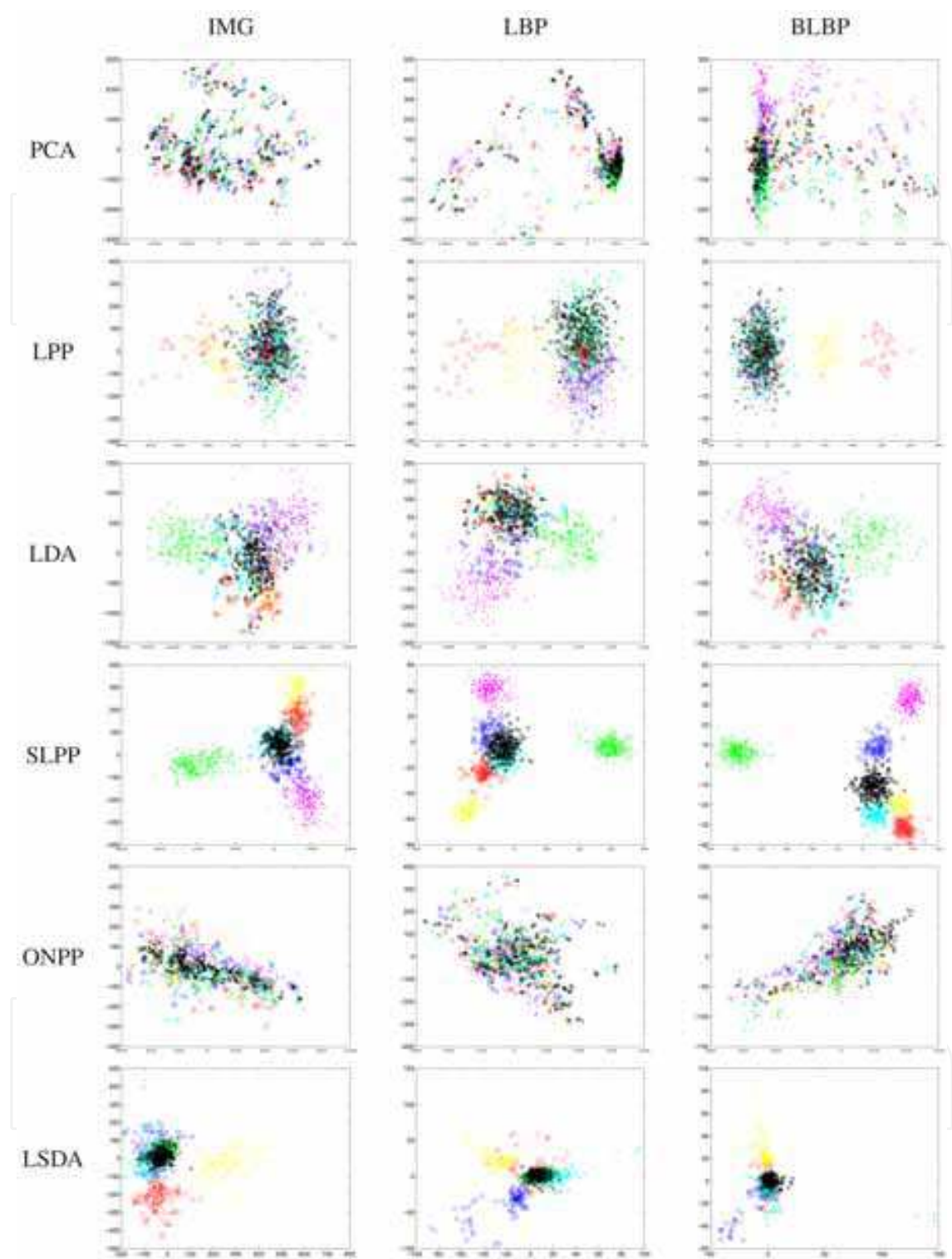
Fig. 9. (Best viewed in color) Images of data set S2 are mapped into 2D embedding spaces. Neutral expression is color coded as black. recognition rates in Fig. 11. On comparing feature representations, it is clearly observed that BLBP features perform consistently better than LBP and IMG features. LBP outperforms IMG most of the time except with LPP, IMG has a slight advantage over LBP.
