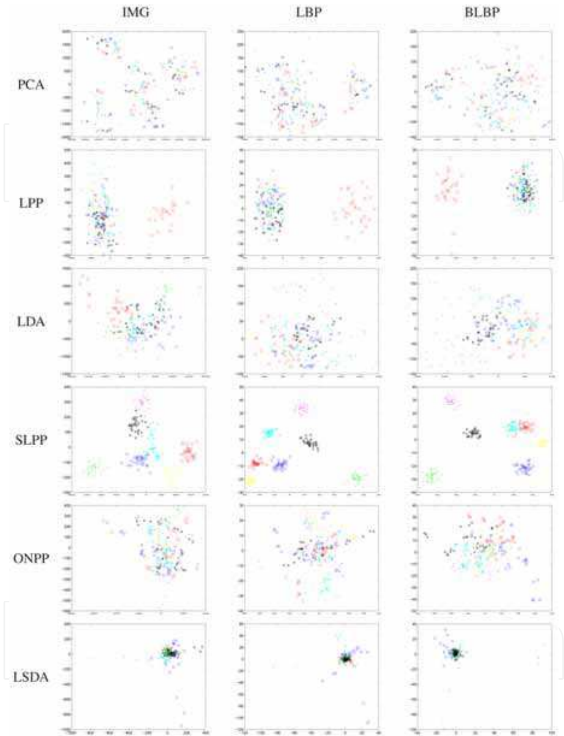
Fig. 17. (Best viewed in color) Images of data set S4 are mapped into 2D embedding spaces. We also plot in the right side of Fig. 18 the averaged recognition rates of different subspace techniques as the function of the reduced dimension when using BLBP features. It is observed the performances of SLPP and LDA become comparable when the reduced dimension increases. On the other hand, ONPP and PCA have similar performance. The plots for S4 shows greater variations compared to those of S1 and S2 (shown in Fig. 12). This may also be due to the small size of the training set.
