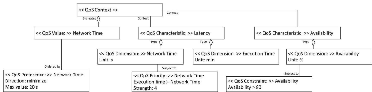
Fig. 6. User specifications
