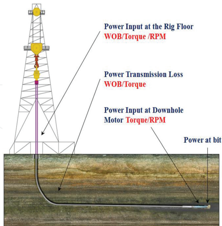
Figure 3. Rotating drilling system with PDM [14].
