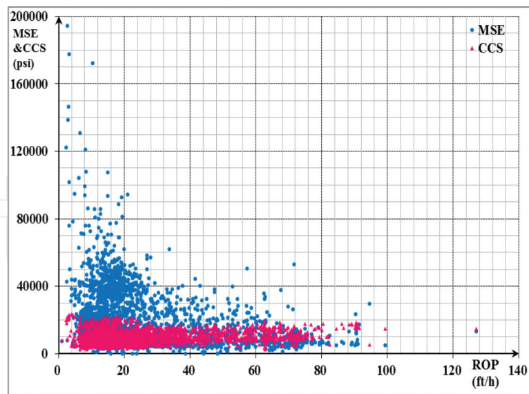
Figure 14. MSE and CCS vs ROP002E.
