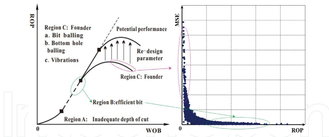
Figure 5. Relationship between the traditional ROP vs. WOB plot and the new MSE vs. ROP plot [12].
