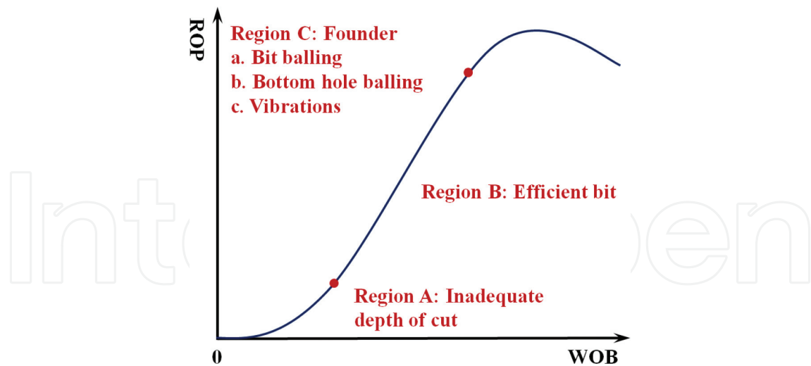
Figure 6. Relationship between the traditional ROP versus WOB plot [14].
