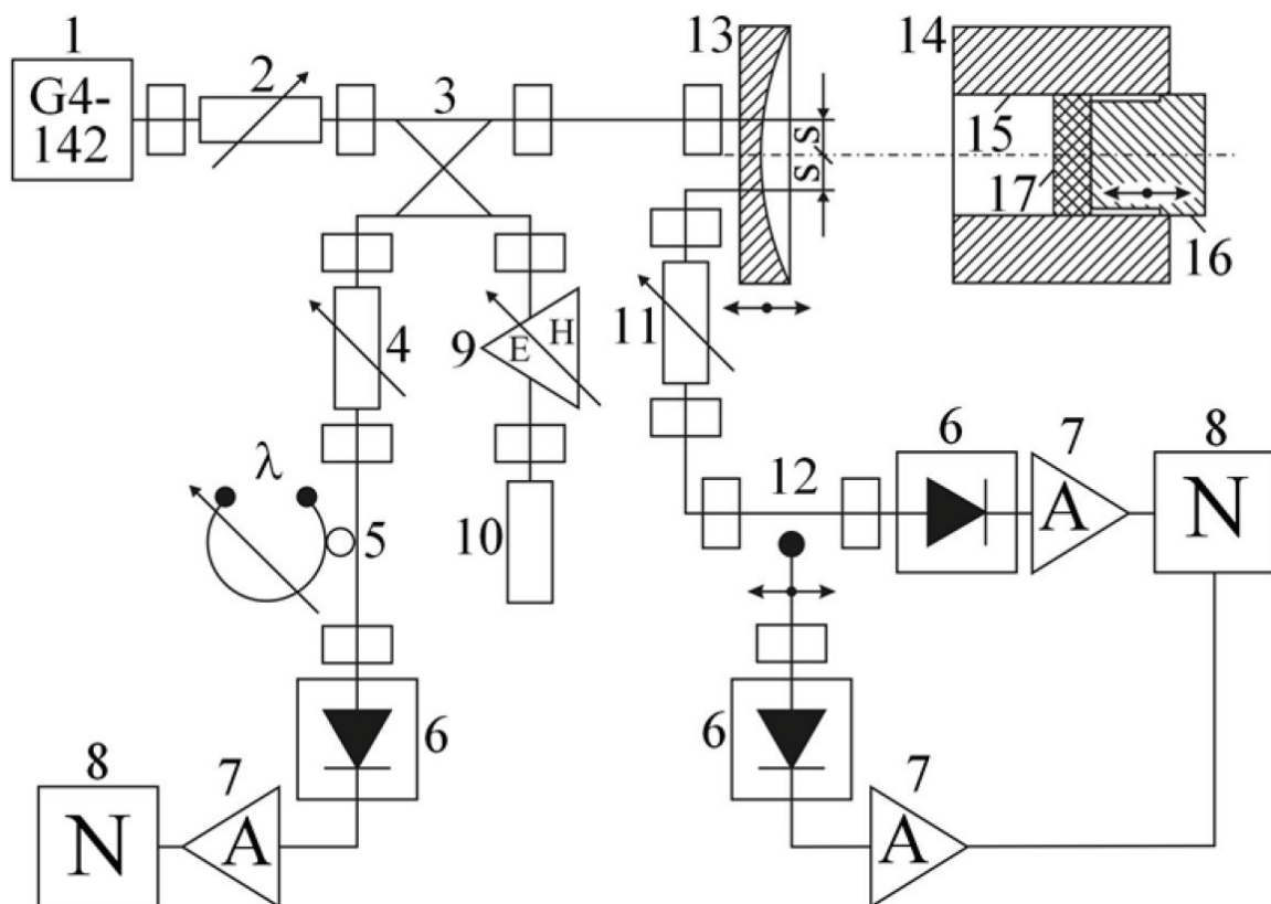
Figure 4. Block diagram of the experimental setup.
