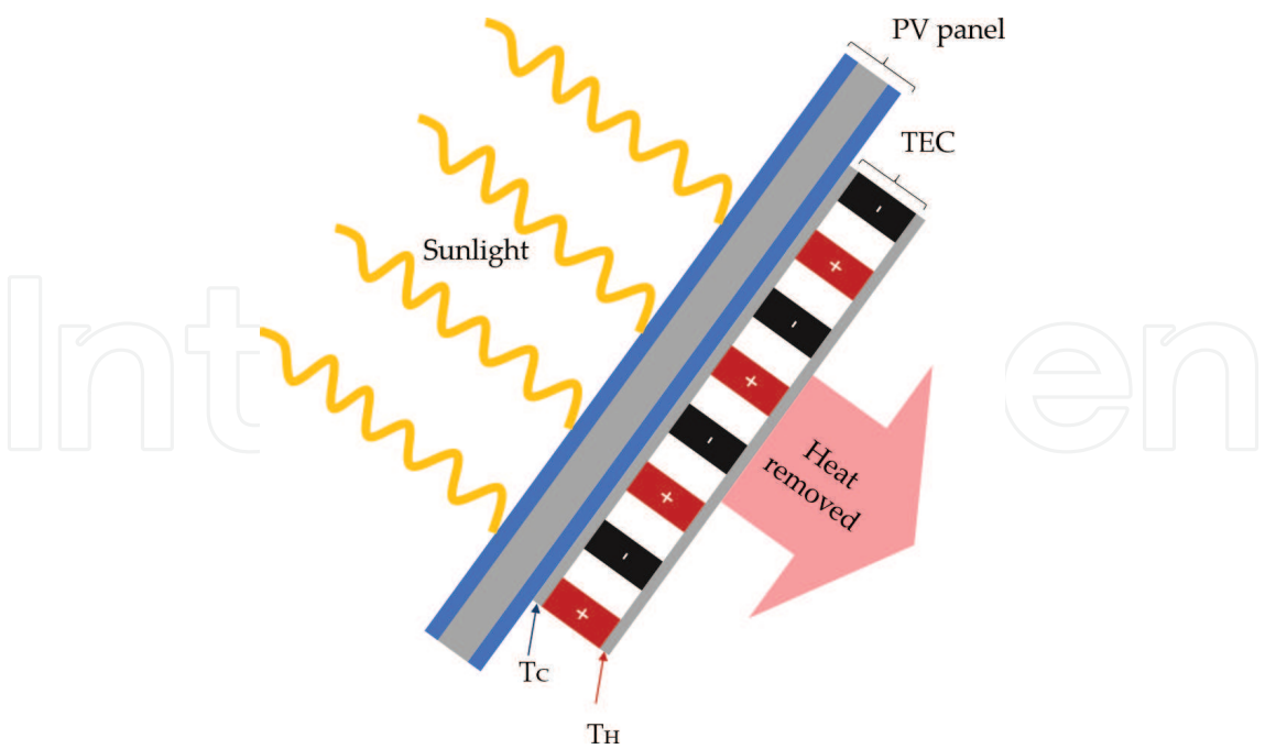
Figure 4. Schematic of the PV+TEC assembly.
