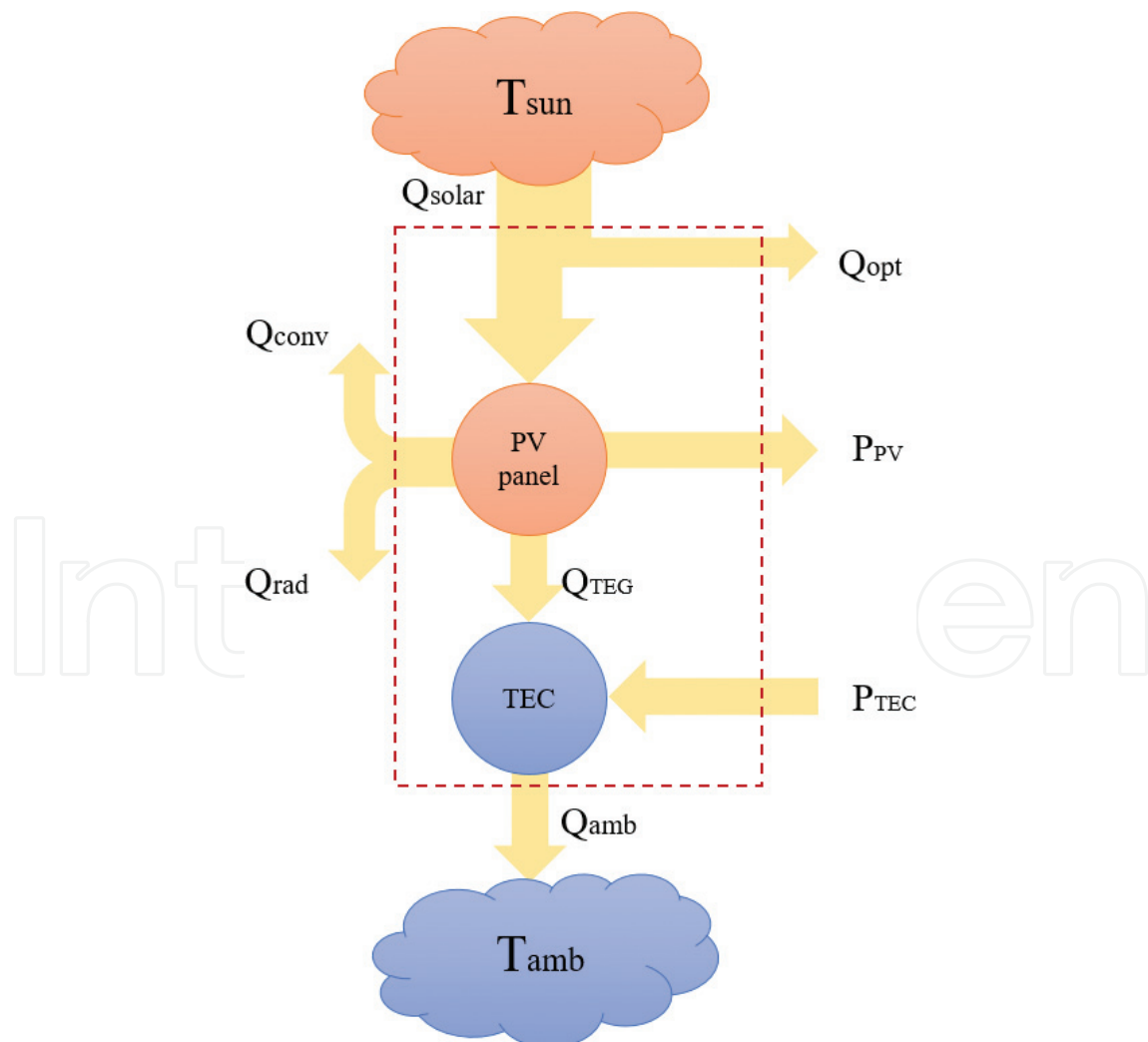
Figure 6. Schematic of the PV+TEC hybrid system limits and energy balance.
