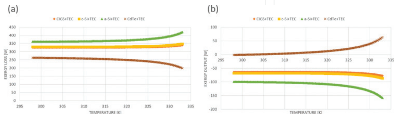
Figure 8. The exergy loss and exergy output for the proposed PV+TEC systems. (a) Exergy loss of PV+TEC systems, (b) Exergy output of PV+TEC systems.
