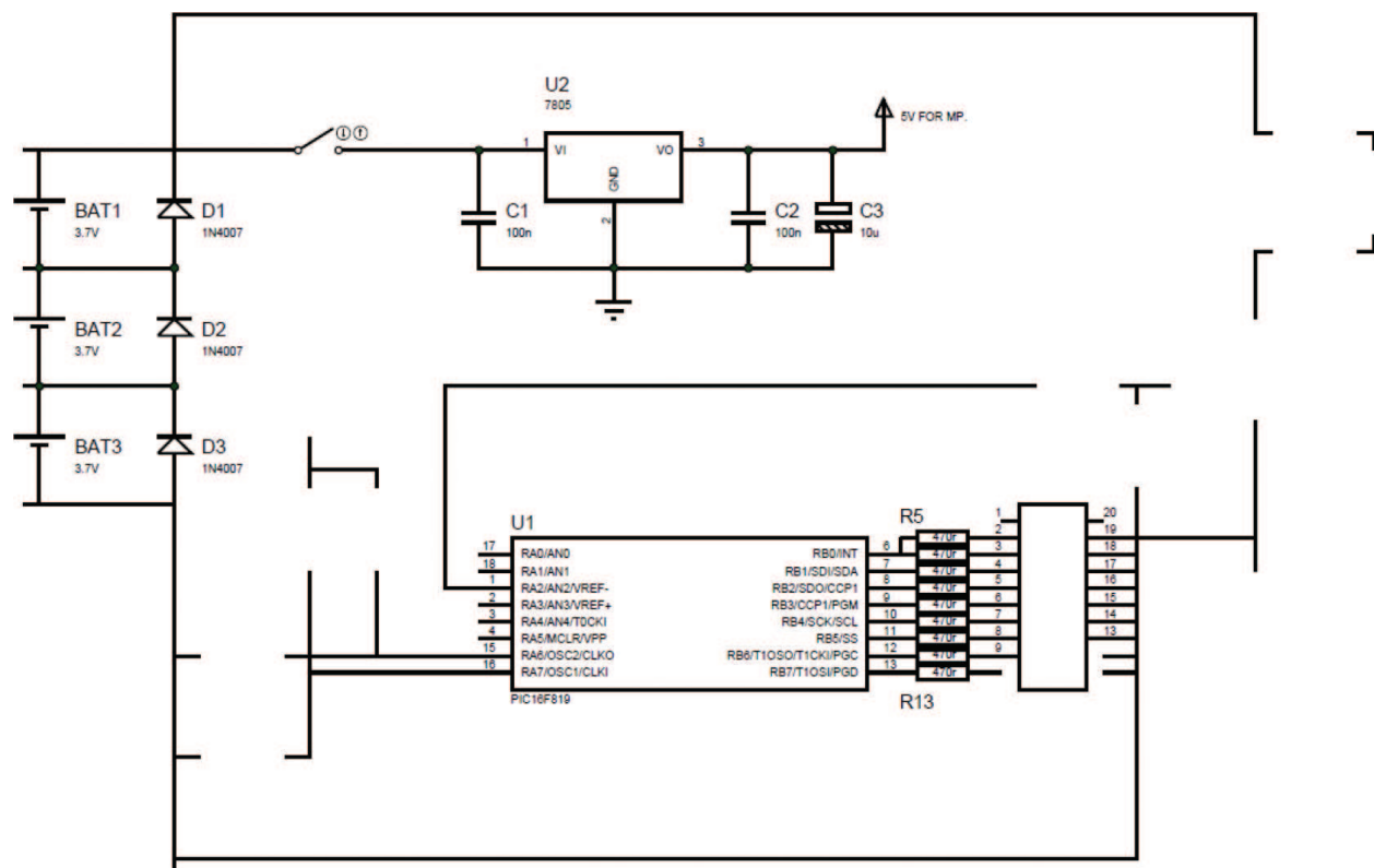
Figure 14. Technical drawing for control module.
