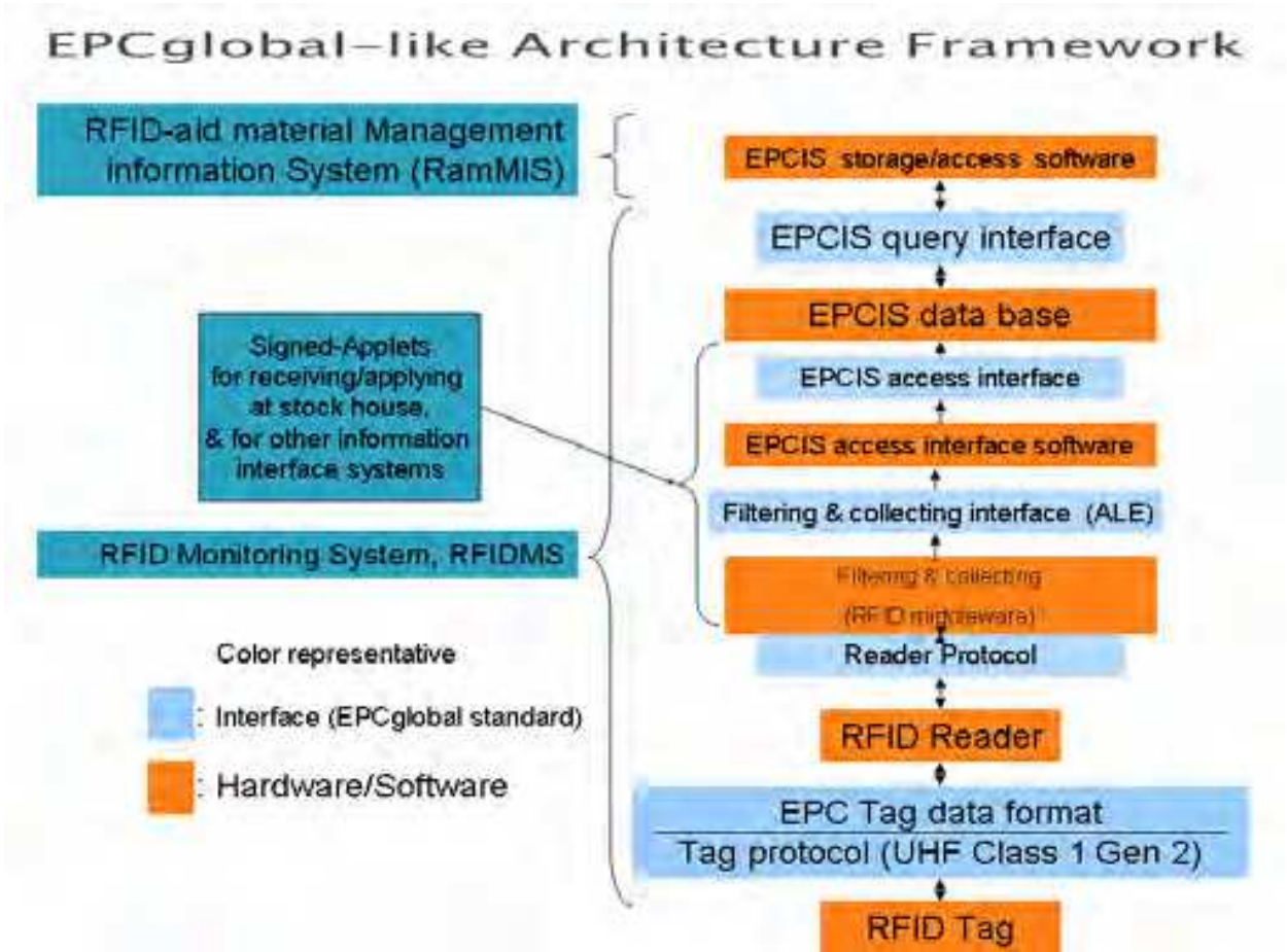
Fig. 4-2. EPCglobal-like Architecture Framework
