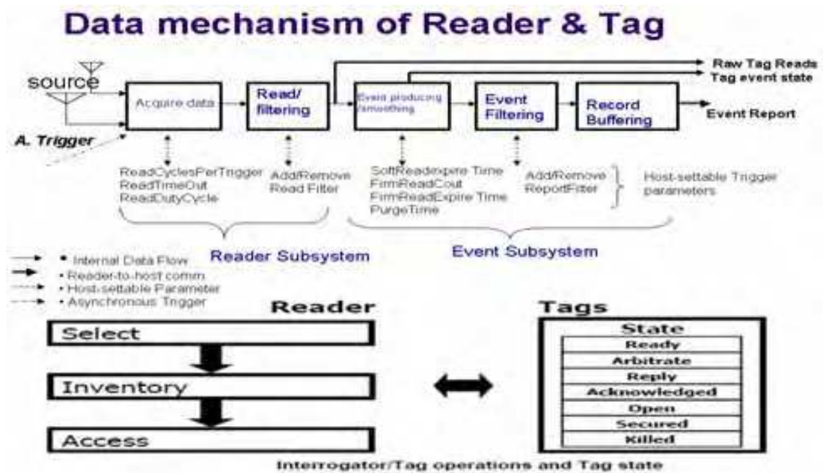
Fig. 2-6. The Data mechanism of reader and tag
