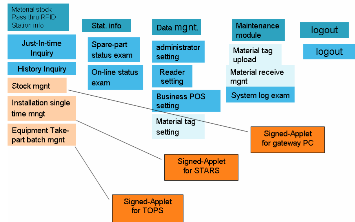
Fig. 4-3. The Functional Structure of RamMIS Website.
