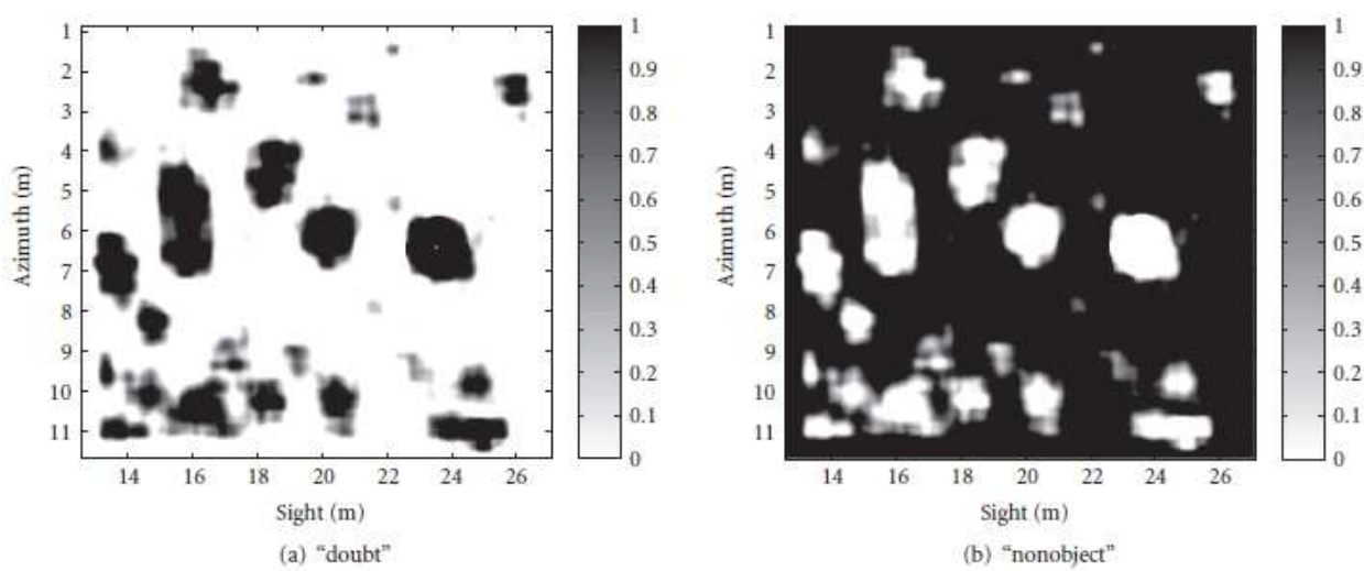
Fig. 26. Mass images obtained for each proposition with the skewness parameter in Fig. 3
