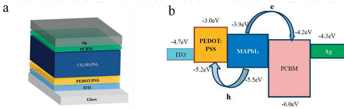
Figure 4. (a) Schematic structure of the devices in this study: \text{ITO}/\text{PEDOT:PSS}/\text{CH}_3\text{NH}_3\text{PbI}_3/\text{PCBM}/\text{Ag} . The thickness of each layer was not in scale with the real thickness for clarity. (b) Schematic illustration of energy band diagram of studied devices (reprinted with the permission from [24], 2016, Elsevier).
