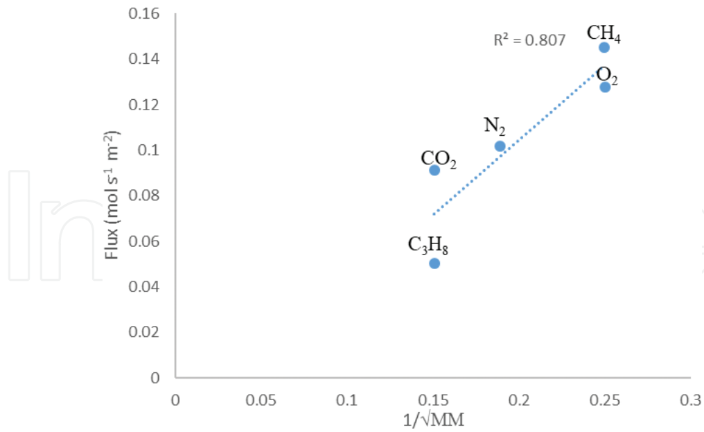
Figure 9. Gas molar flux against the inverse square root of molecular weight.
