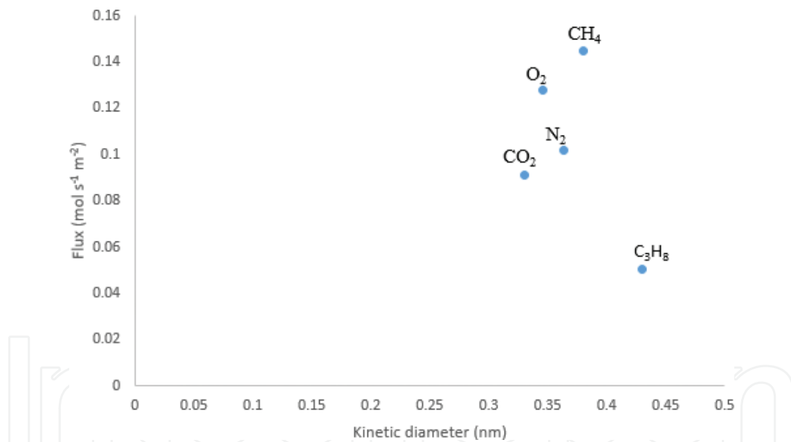
Figure 10. Gas molar flux against kinetic diameter of gases.
