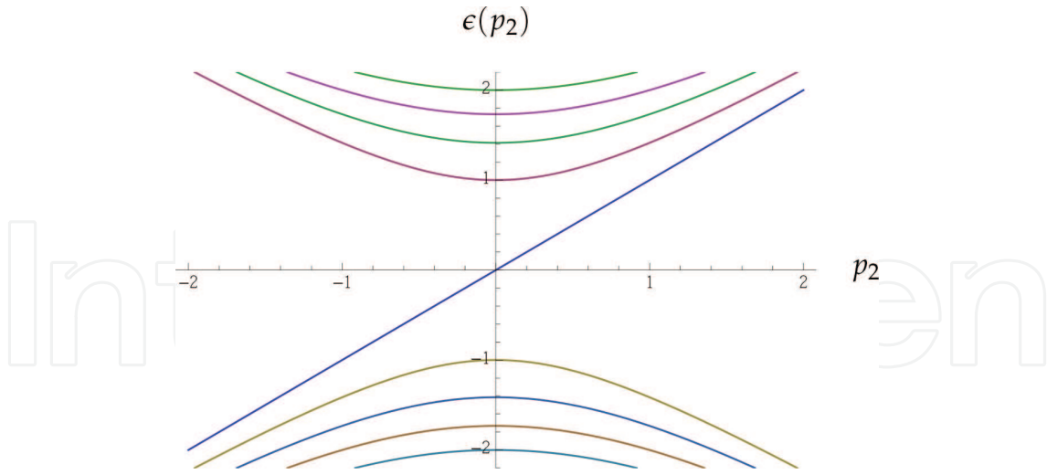
Figure 3. The dispersion relation of the edge state with \vartheta = 1 . We find a gapless chiral mode specific to the 2d class A TI. The gapped spectra are interpreted as bulk contributions.
