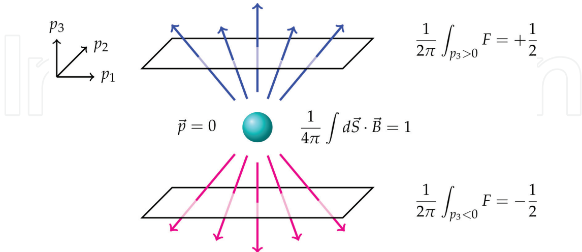
Figure 1. Monopole at Weyl point in the momentum space. The monopole charge is an integer-valued topological invariant \nu_{3d} . The 2d invariant \nu_{2d} is obtained at a constant p_3 (\rightarrow m) plane, which covers either upper or lower half of the fluxes, so that \nu_{2d} is given by a half of \nu_{3d} .
