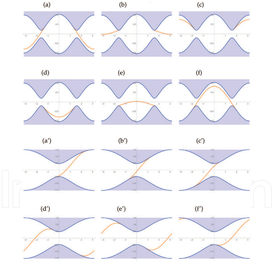
Figure 10. The boundary condition dependence of the 2d lattice system (52) and (53) with c = 1 . (a)–(f) and (a')–(f') show the spectra obtained from the reduction p_1 \rightarrow m_1 = \pi/2 + 0.5 and p_2 \rightarrow m_2 = 0.2 . The horizontal axes are the momenta p_2 and p_1 , respectively. The blue region is the bulk, and the orange line is the edge state spectrum.
