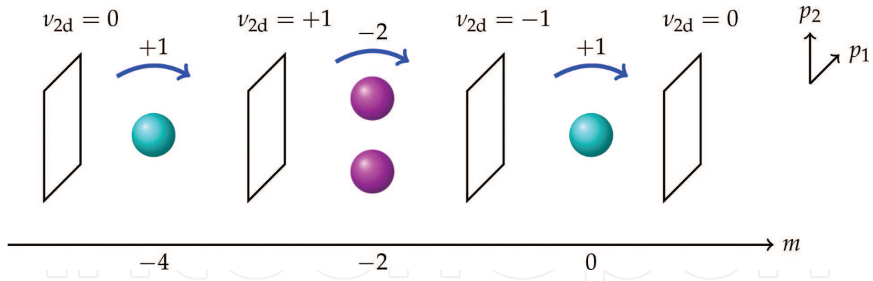
Figure 4. The mass dependence of the 2d topological invariant v_{2d} for the lattice model (10). Topology change occurs at the gapless points m = -4, -2, 0 . Change of the invariant corresponds to the monopole charge +1, -2, +1 associated with each gapless point.
