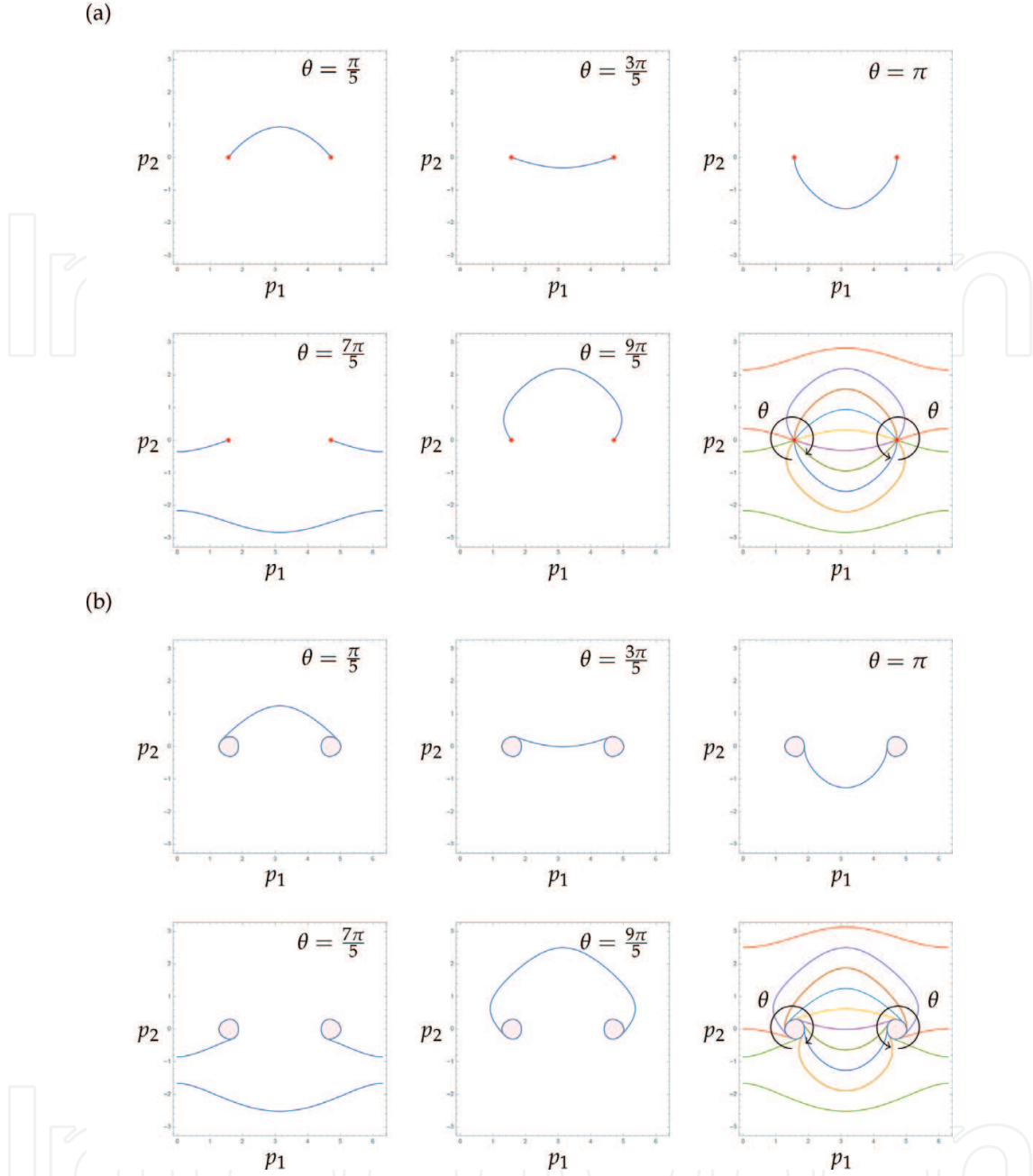
Figure 8. The Fermi arc at (a) zero energy \varepsilon(\vec{p}) = 0 and (b) finite energy \varepsilon(\vec{p}) = 0.3 with \theta = \pi/5, 3\pi/5, \pi, 7\pi/5, 9\pi/5 . The red dot and shaded region show the bulk contribution. The last panels show Fermi arcs with various values of the parameter \theta .
