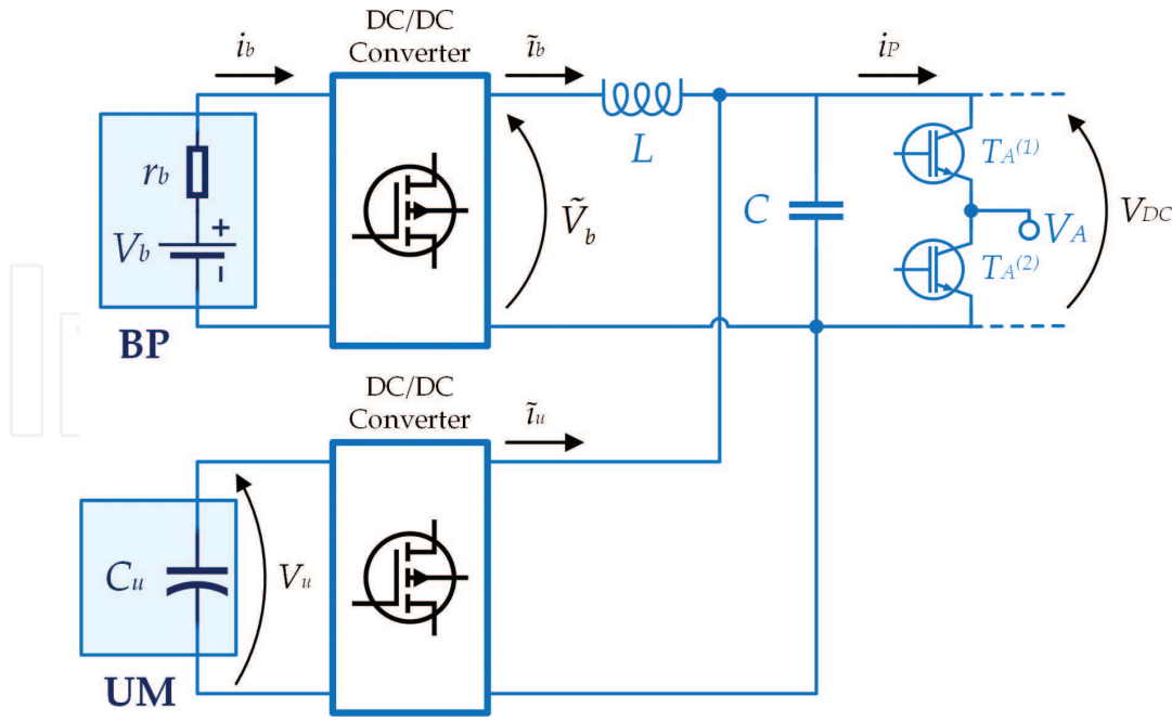
Figure 4. Schematic representation of active parallel HESS configuration.
