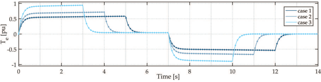
Figure 12. Motor torque evolution achieved over vehicle start and stop.
