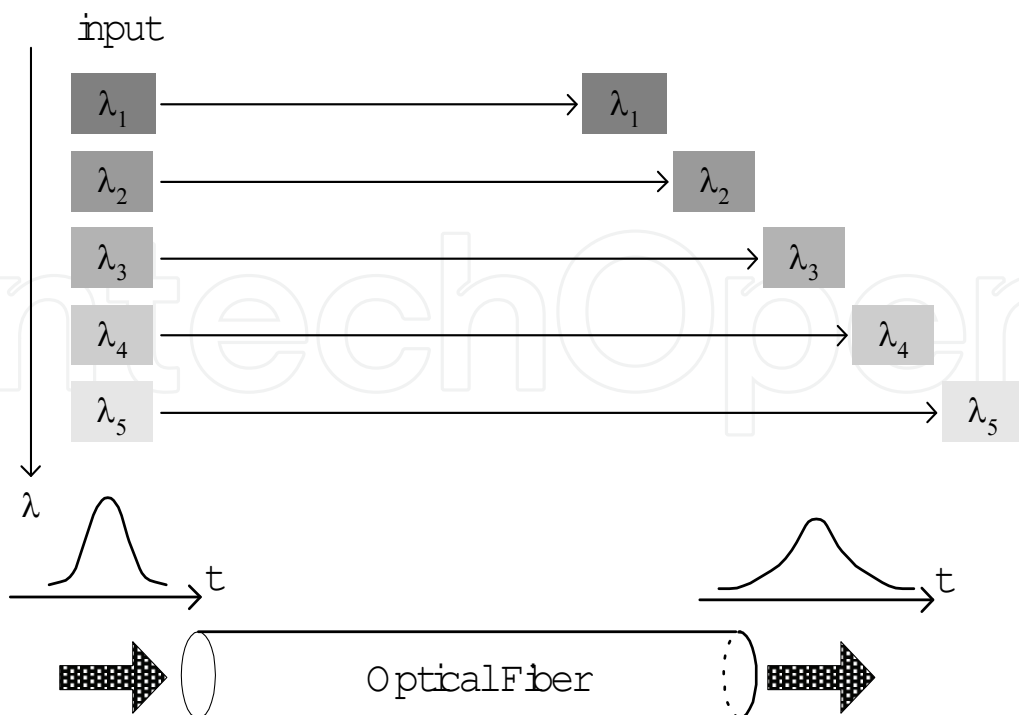
Fig. 2. Schematic diagram of chromatic dispersion.
