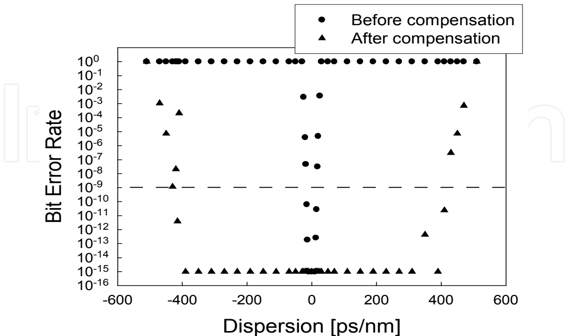
Fig. 10. Compensation range of the proposed method at 40 Gb/s.
