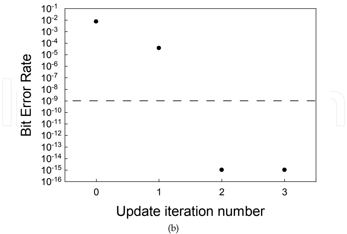
Fig. 8. BERs at every update of the compensator (a) 0→20km, (b) 20→25km.
