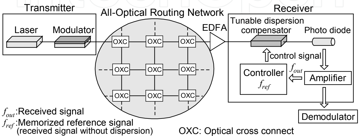
Fig. 6. Schematic diagram of all-optical dynamic routing network with the adaptive dispersion compensation technique.
