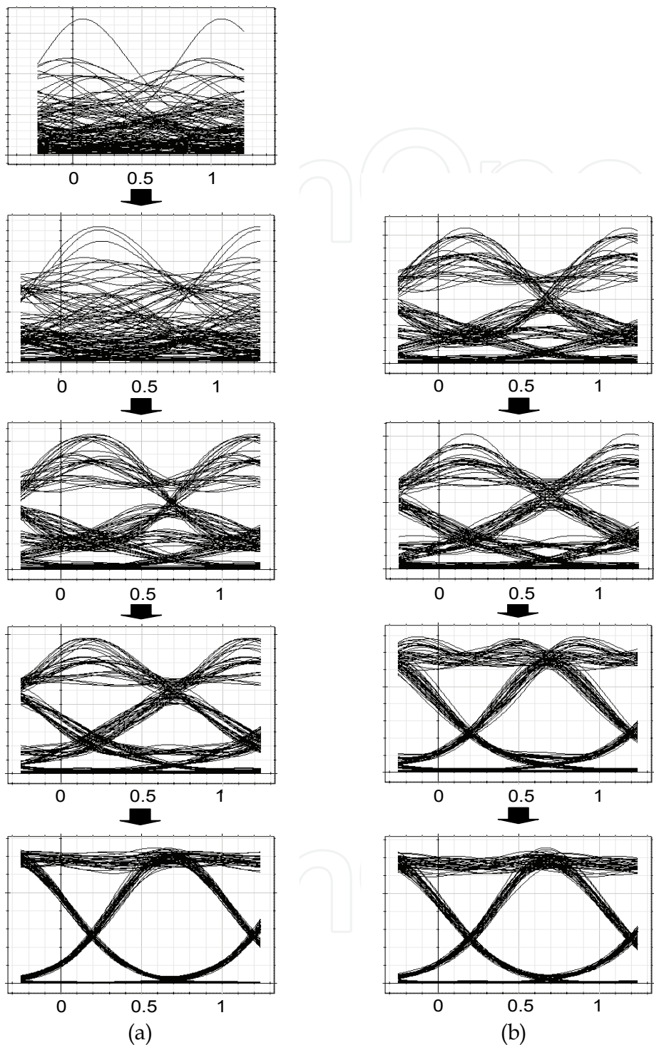
Fig. 9. Eye-diagrams at every update of the compensator (a) 0→20km, (b) 20→25km.
