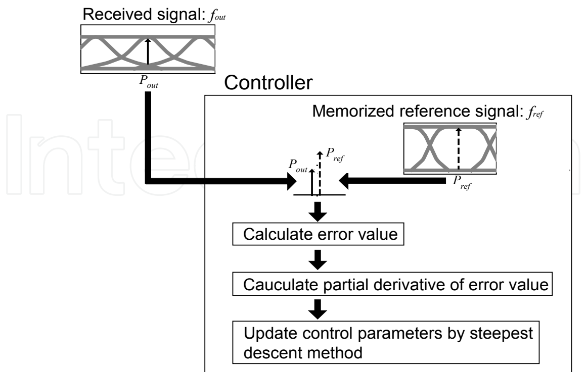
Fig. 7. Procedure of proposed steepest-descent-based control.
