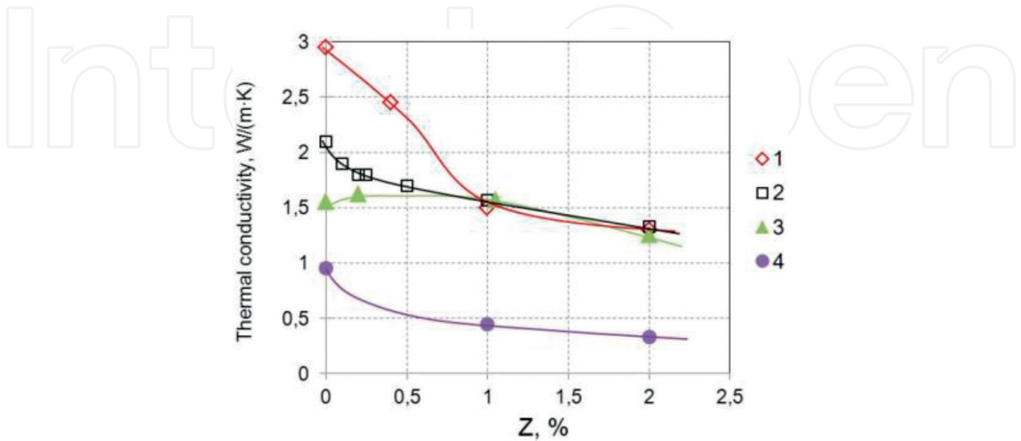
Figure 3. Salinity (Z,%) dependence of thermal conductivity for different types of NaCl-bearing soil: 1—fine sand, 2—silty sand, 3—sandy clay, and 4—kaolin clay (W = 15–30% for 1–3 and W = 50–70% for 4) [18]. Data points are experimental measurements; lines are approximation trends.
