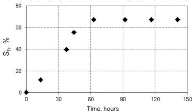
Figure 5. Pore hydrate formation in gas-saturated silty sand ( W = 18\% ; n = 0.40 ), at t = +2 \pm 1^\circ\text{C} : time-dependent hydrate saturation ( S_{\text{h}} , %) [45].
