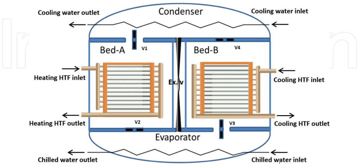
Figure 9. Schematic diagram of a conventional two-bed adsorption chiller, as Bed-A in desorption mode, Bed-B in adsorption mode.
