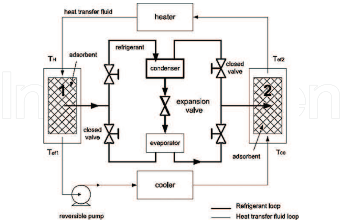
Figure 10. Schematic representation of the thermal wave adsorption heat pump during the first half of the cycle [63].
