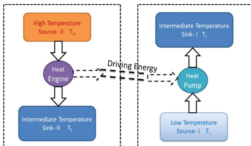
Figure 1. Representation of the thermodynamics cycle of ideal ARS.
