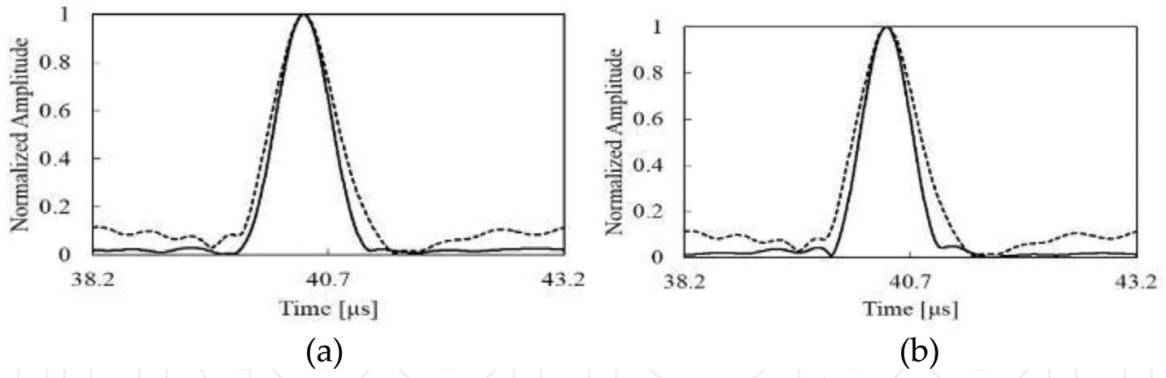
Figure 12. Normalized envelope signal of compressed fundamental echo obtained by simulation before FDA compensation (dashed line) and after FDA compensation (solid line): (a) with linear FDA approximation and (b) with nonlinear FDA approximation.
