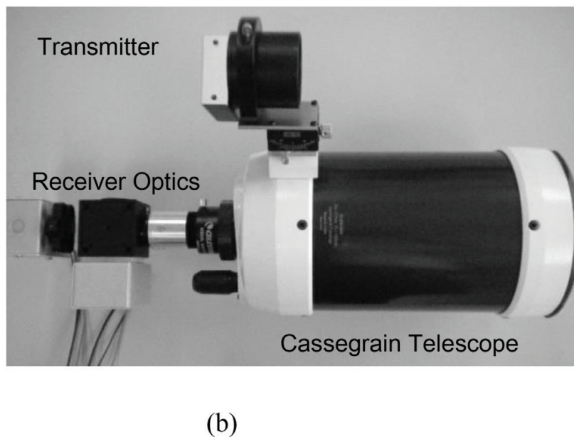
Figure 8. LED mini-Raman lidar. (a) Optical structure. (b) Lidar setup.
