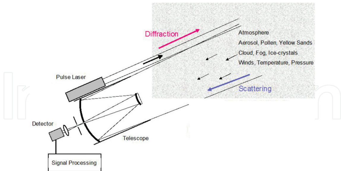
Figure 2. Lidar principle.
