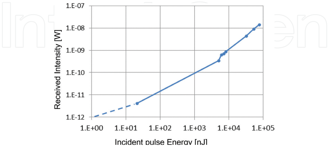
Figure 7. Raman scattering echo detection with lowered incident power.
