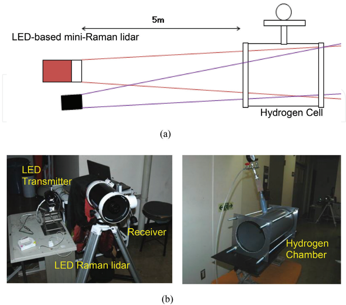
Figure 10. Hydrogen gas quantitative measurement. (a) Quantitative measurement of hydrogen gas. (b) System setup and arrangement.
