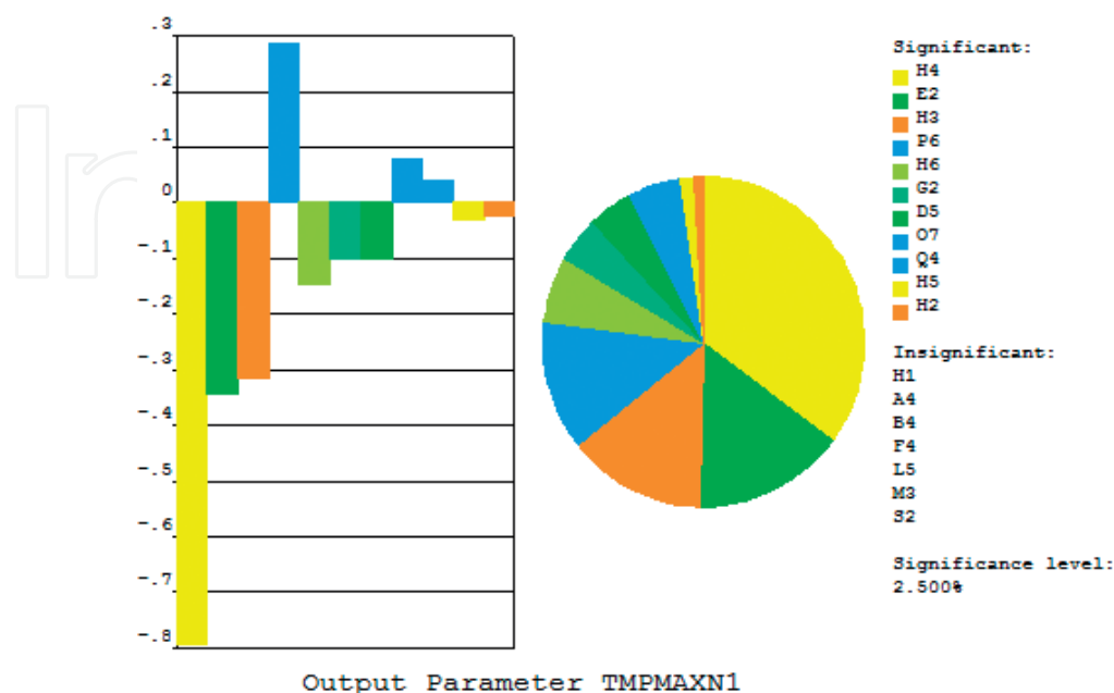
Figure 12. Sensitivity of maximum bondline temperature to random input parameters.
