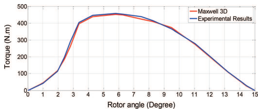
Figure 15. Comparison of Maxwell 3D and experimental results.
