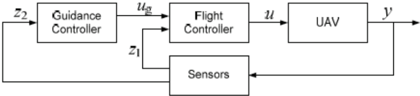
Figure 4. UAV recovery control diagram
