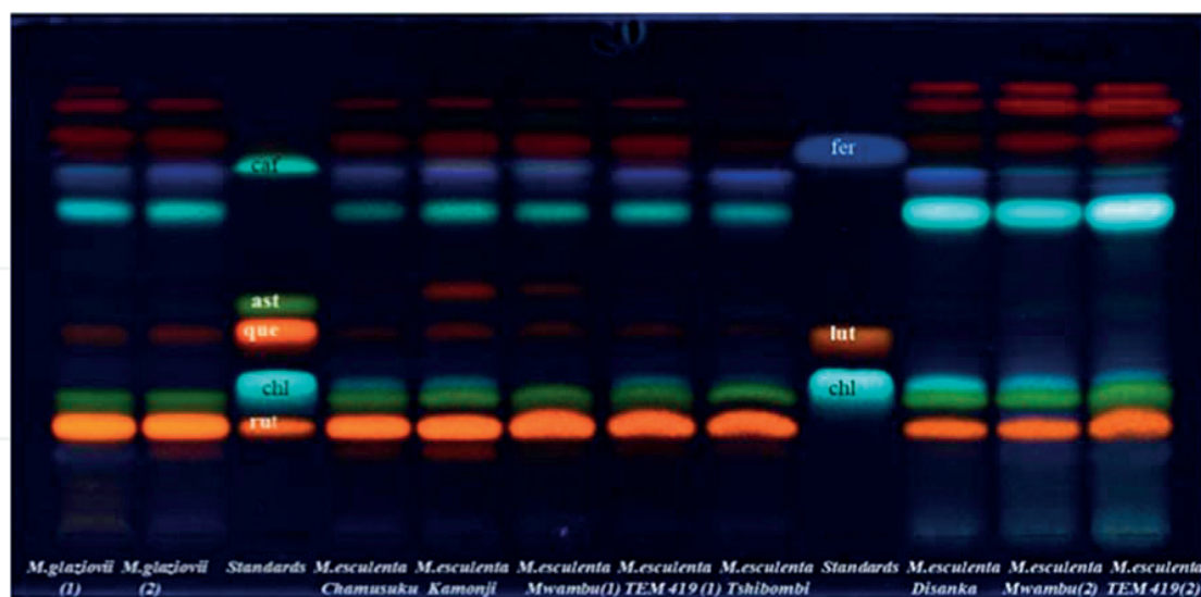
Figure 3. TLC chromatogram of methanolic extracts from M. esculenta (varieties: Chamusuku , Disanka , Kamonji , Mwambu , Tshibombi , TEM 419 ), M. glaziovii with astragalin (ast), caffeic acid (caf), chlorogenic acid (chl), ferulic acid (fer), luteolin(lut), quercitrin(que) and rutin (rut) as standards; developed with ethyl acetate/formic acid/methanol/water (20:0.5:2.5:2; v/v/v/v) and visualized at 365 nm with natural products-PEG reagent. Flavonoids are detected as yellow-orange fluorescent spots and phenolic acids as blue fluorescent spots.
