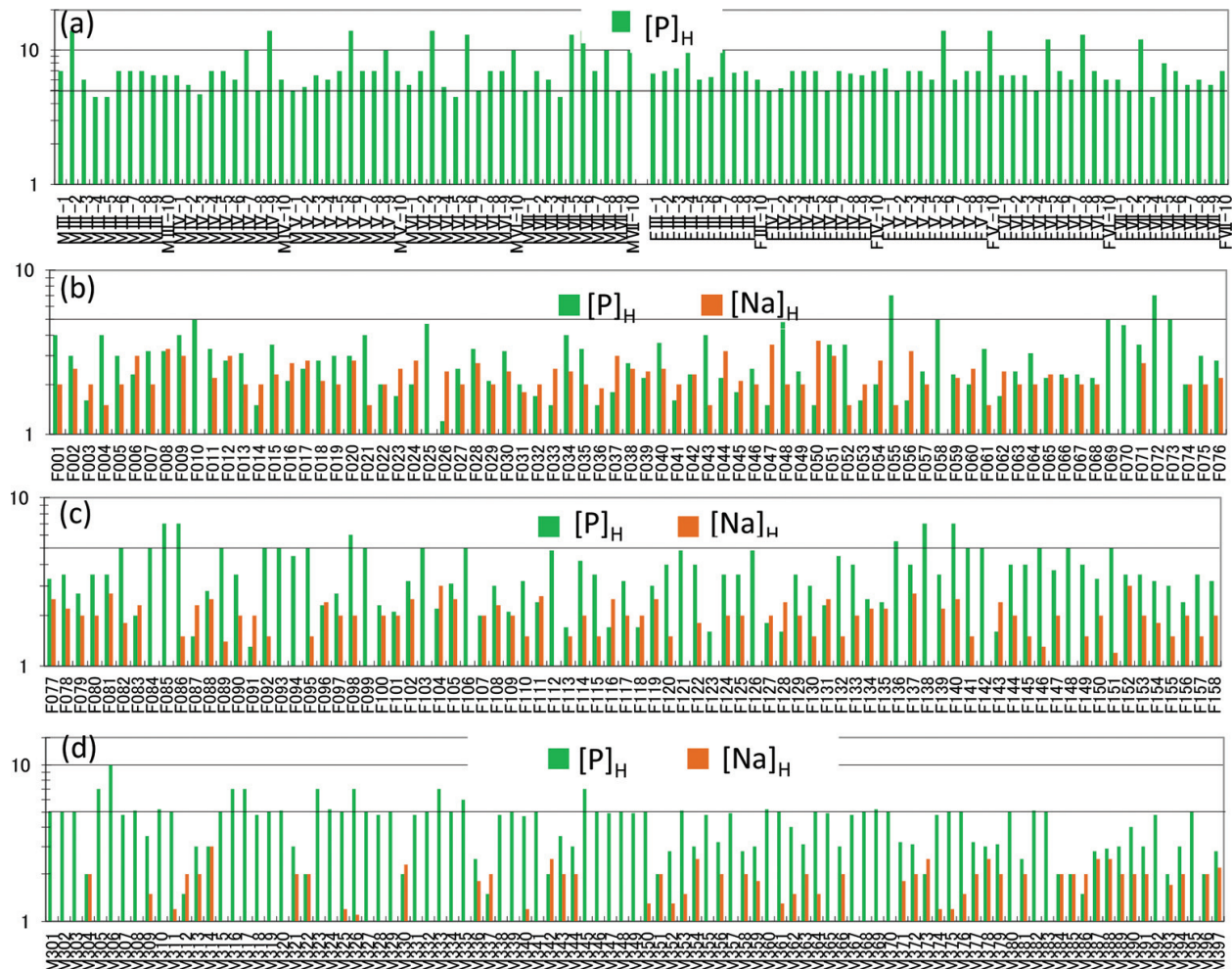
Figure 7. Association between [P]_H and [Na]_H with inactive Na^+/K^+-ATPase due to the air pollution. (a) [P]_H without air pollution for the male and female subjects in Figure 3 . The upper and lower levels are seen at [P]_H \geq 10 and [P]_H = 5 , respectively. [Na]_H is not seen by the normal Na^+/K^+-ATPase . (b) and (c) show [P]_H and [Na]_H for the female subjects in Figures 4 and 5 , respectively. [P]_H lower than the usual lower level is seen with the appearance of [Na]_H peak. (d) [P]_H for the male subjects in Figure 6 ; the low [P]_H is accompanied by the [Na]_H peak. The low [P]_H values are often seen for the male over 60 (M351: 63). The abnormally low [P]_H indicates insufficient energy supply to the Na^+/K^+-ATPase . Breathing the polluted air increases serum [Ca^{2+}] which moves to bone, accompanied by P to cause P deficiency.
