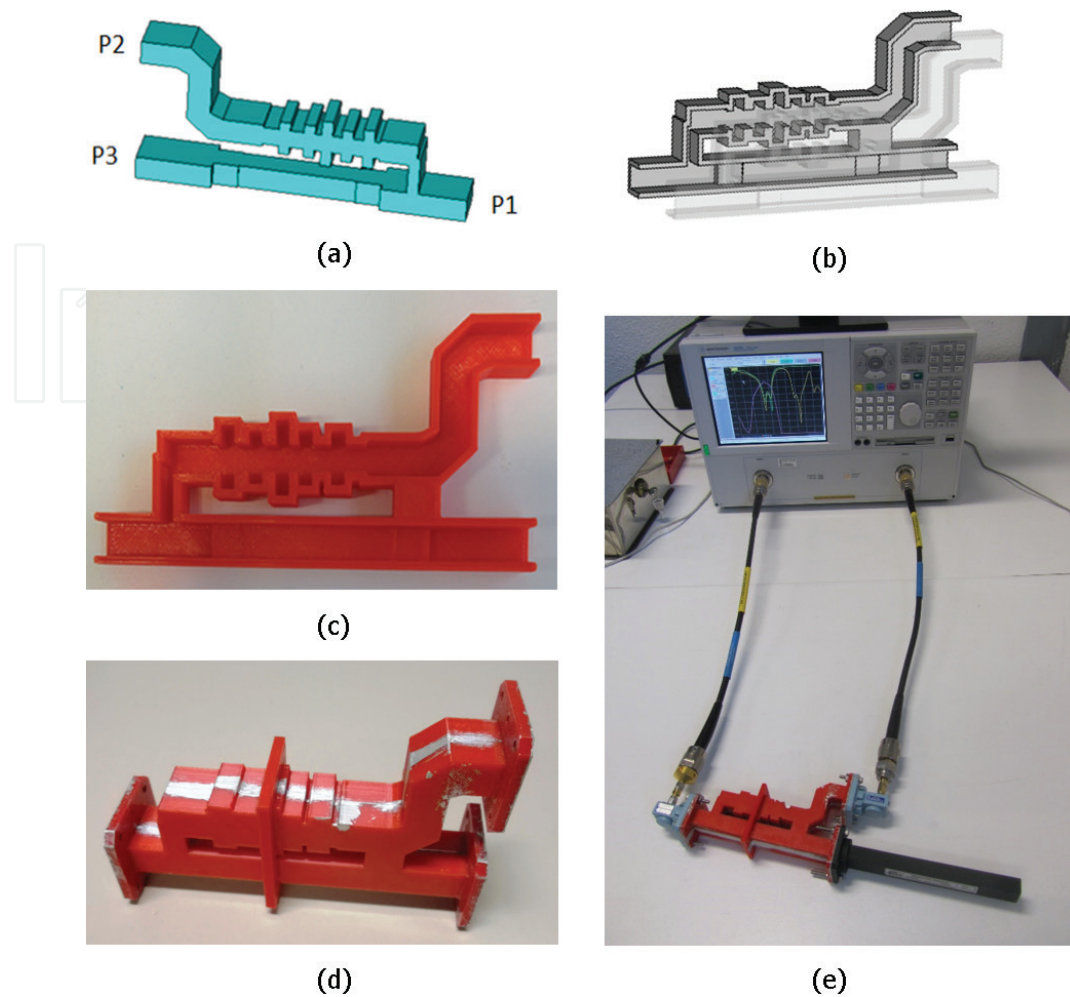
Figure 21. (a) Diplexer layout, (b) half CAD model, (c) one printed half, (d) the device metallized and assembled, and (e) measurement setup.
