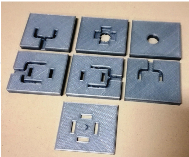
Figure 4. Printed layers of an ortho-mode transducer (OMT) based on turnstile junction, working in W-band.
