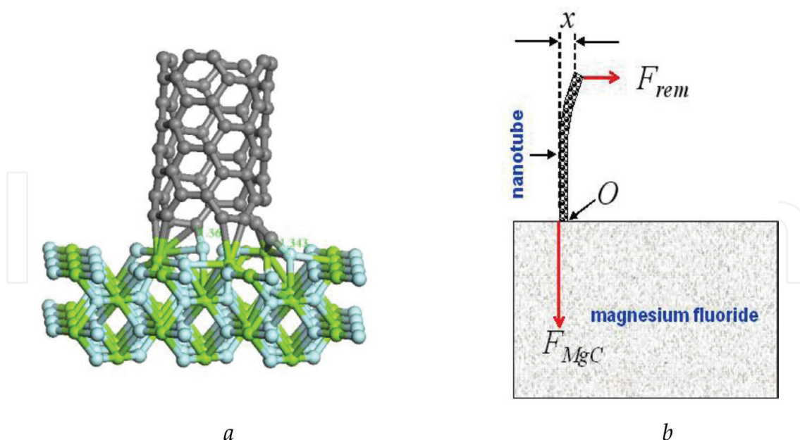
Figure 2. Possible covalent bonding formation in the systems of MgF 2 -CNTs (a) [24] and analytical calculation of this process (b) [25].
