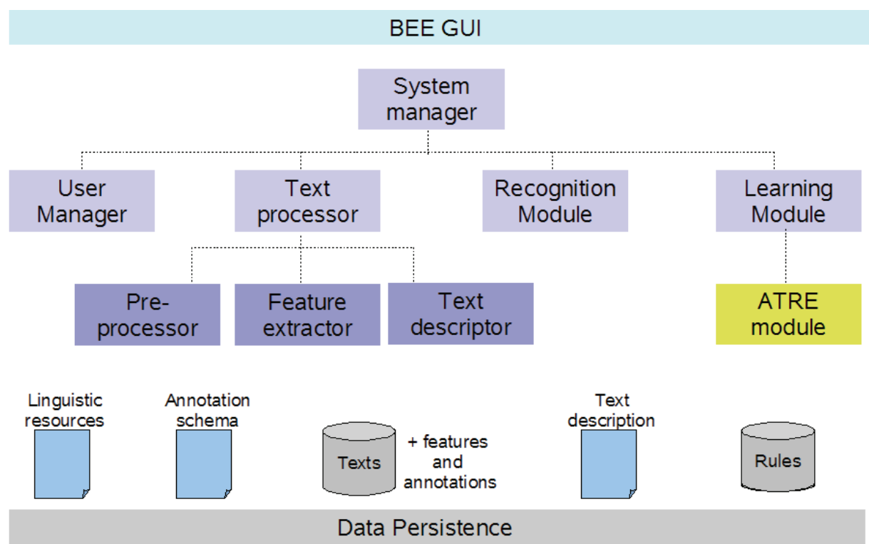
Fig. 2. BEE architecture
