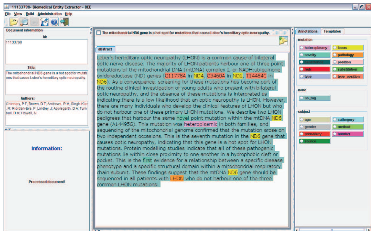
Fig. 1. BEE GUI
