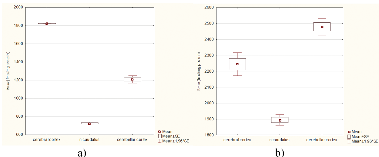
Figure 20. Statistical analysis of [^3\text{H}] PK-11195 binding parameters [ B_{\text{max}} (fmol/mg of protein) – density of binding sites] with mitochondrial membranes in different areas of the human brain in control group (a) and study group (b) (alcoholic patients).
