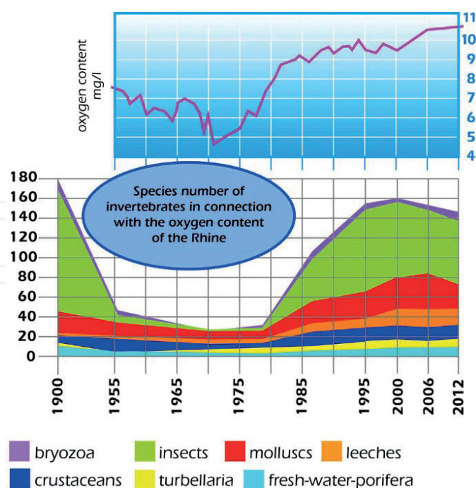
Figure 9. Development of the invertebrate communities of the Rhine and average oxygen content of the Rhine at Emmerich (Lower Rhine).
