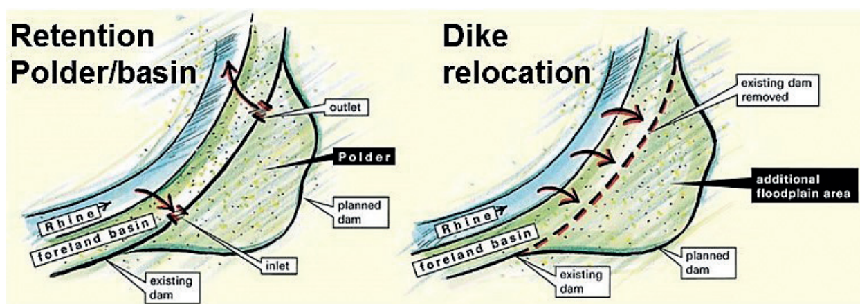
Figure 17. Example of measures aimed at lowering water levels: retention basin and dike relocation (source: Regierungspräsidium Freiburg—Integrated Rhine Programme (2011)).
