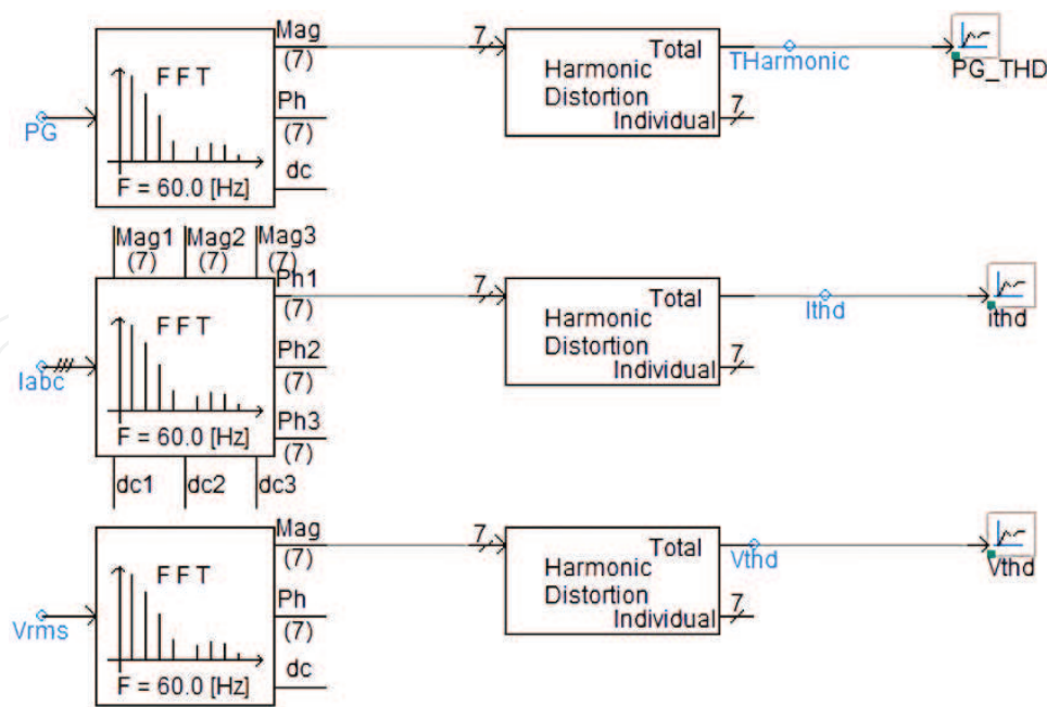
Figure 3. PSCAD modeling of 7th order 60 Hz for THD of active power, current, voltage at the PCC.
