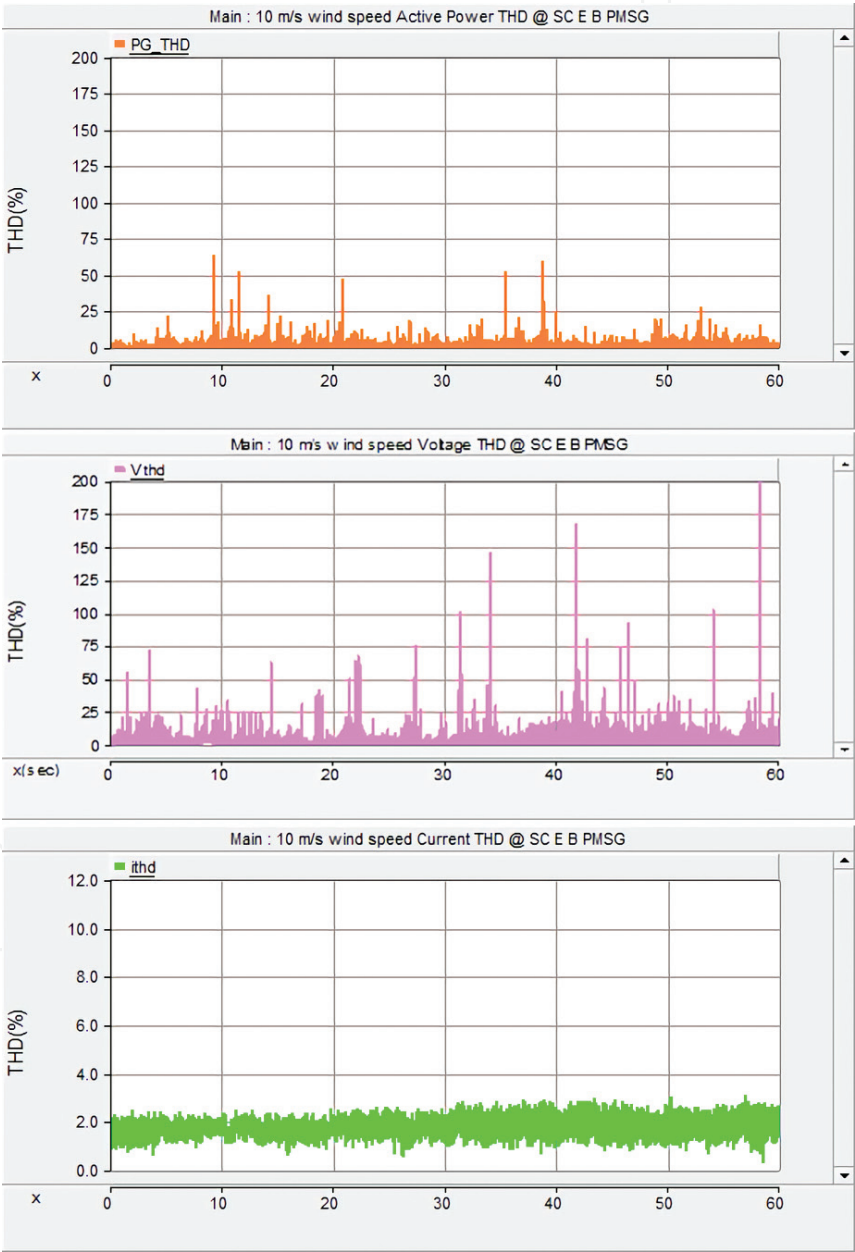
Figure 10. THD (%) of HYEES PMSG during 60 sec: active power THD of B-SC-E ESS, current THD of B-SC-E ESS, voltage THD of B-SC-E ESS.
