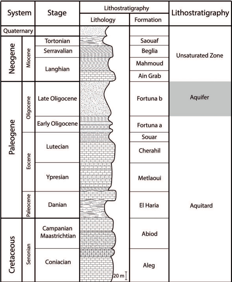
Figure 2. Simplified lithostratigraphic column of the study areas.
