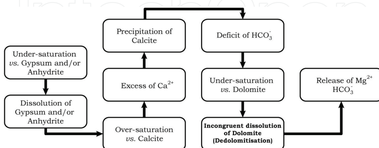
Figure 7. Schematic model showing the dedolomitization process.
