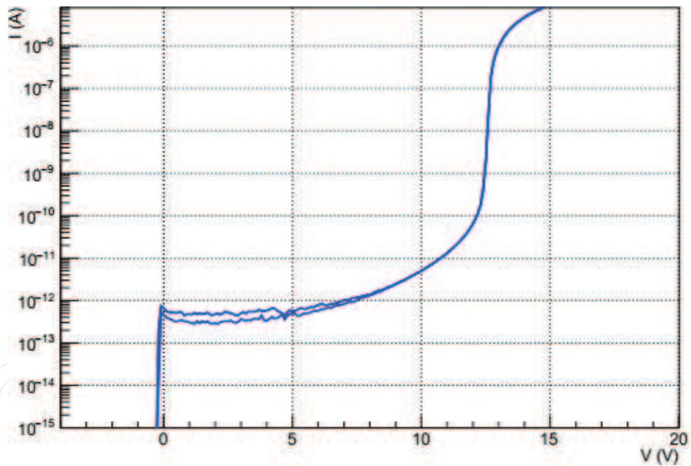
Figure 11. Current-voltage characteristics of structure II.
