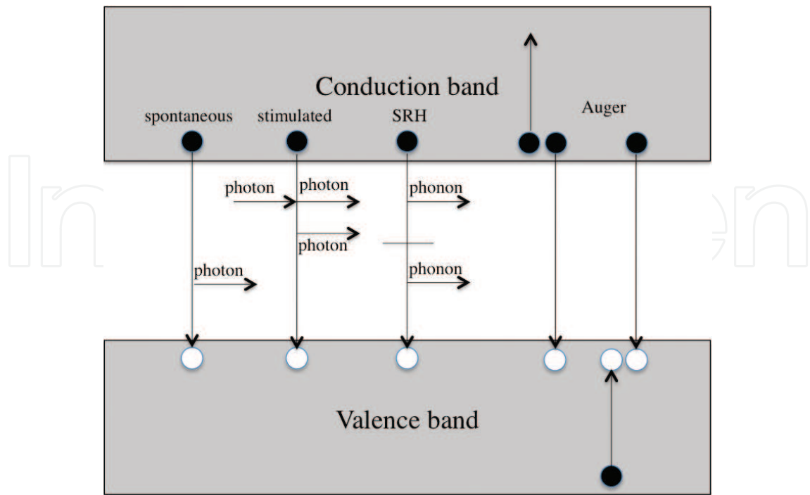
Figure 4. Radiative and non-radiative recombination processes in semiconductor devices.
