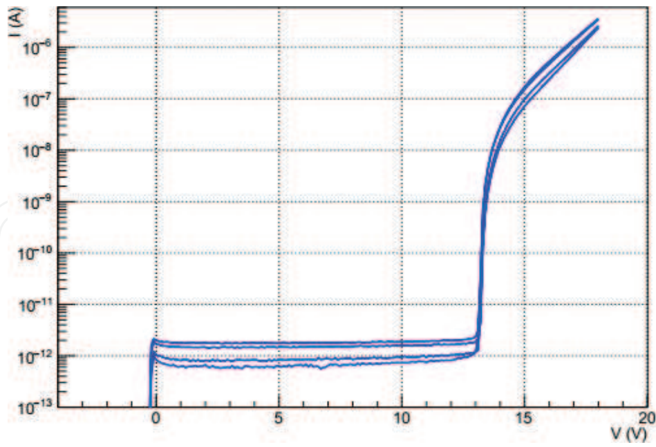
Figure 10. Current-voltage characteristics of structure I.
