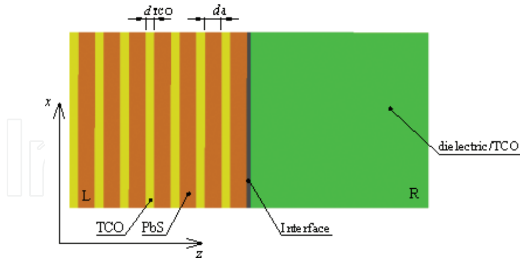
Figure 1. One-dimensional MM composed of alternating TCO and dielectric layers. The MM/dielectric ( \epsilon_R = 1 or \epsilon_R = 2.25 ) and MM/TCO interfaces are considered.
