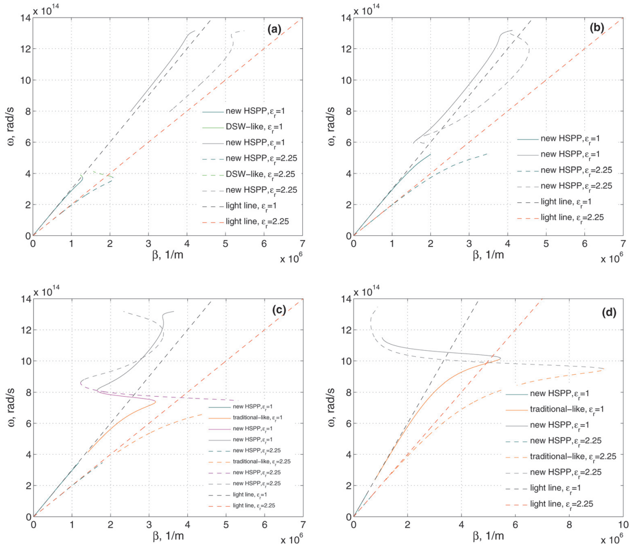
Figure 4. Dispersion curves of HSPPs for various TCO-filling ratios, i.e. f_{\text{TCO}} = 0.3 in (a), f_{\text{TCO}} = 0.5 in (b), f_{\text{TCO}} = 0.7 in (c) and f_{\text{TCO}} = 0.9 in (d), corresponding to the MM/dielectric interface.
