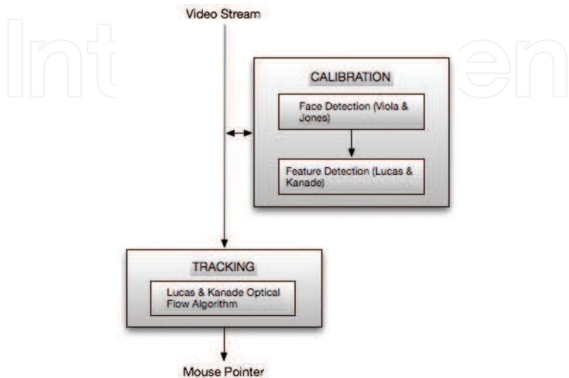
Fig. 4. The head-tracking component. After initial calibration, the video stream is processed in real-time by the tracking algorithm.
