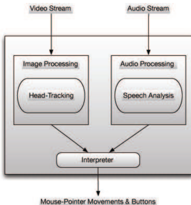
Fig. 1. High-level system overview.
