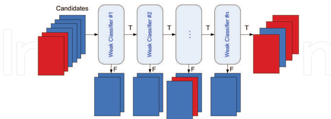
Fig. 3. Weak classifiers are arranged in a cascade. Note that some incorrect classifications may occur, as indicated in the diagram.
