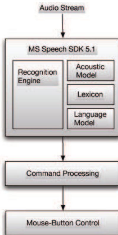
Fig. 7. The speech-recognition components of our head-tracking system.
