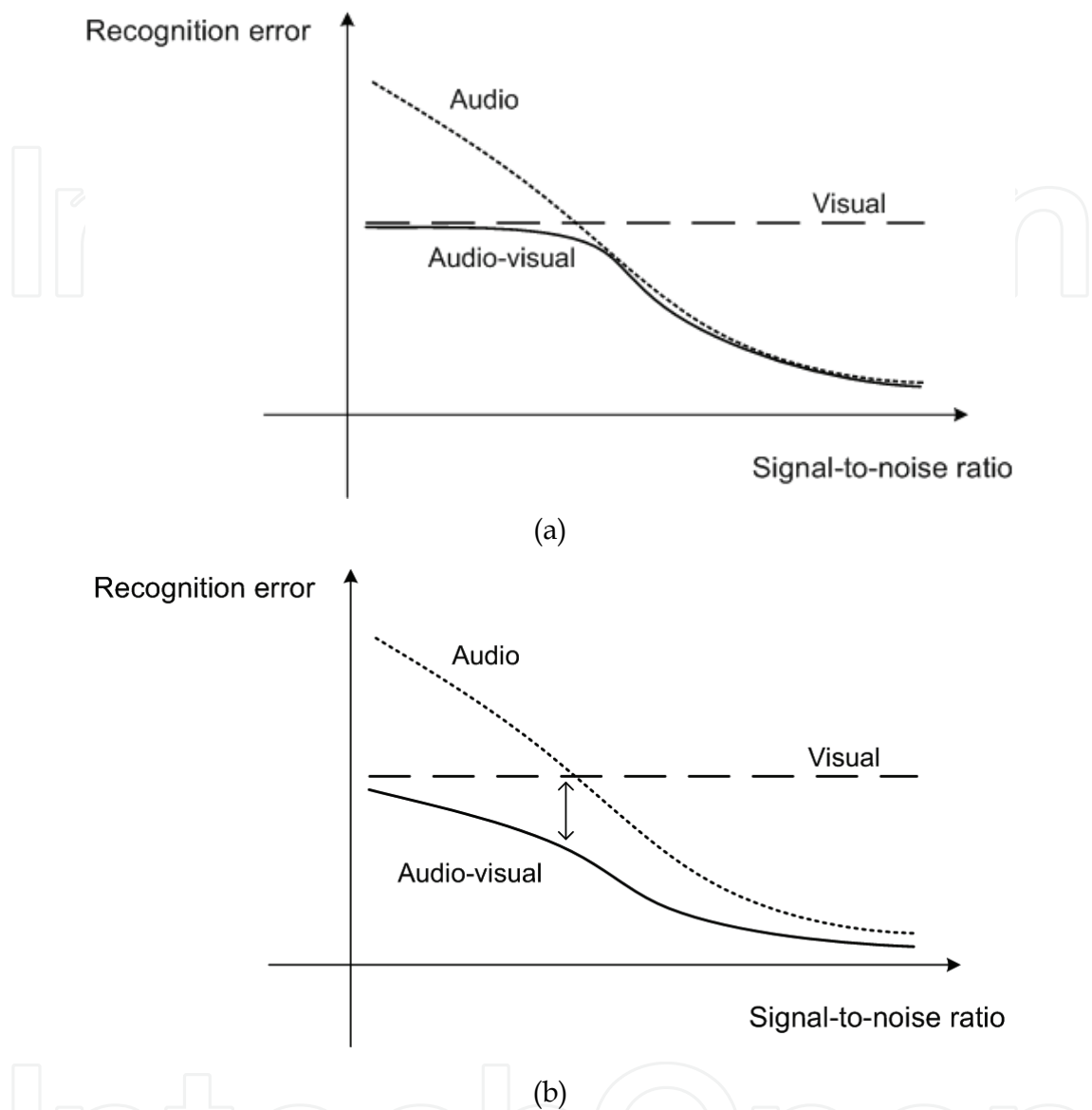
Fig. 3. Two challenges of AVSR. (a) The integrated performance is at least that of the modality showing better performance for each noise level. (b) The integrated recognition system shows the synergy effect.
