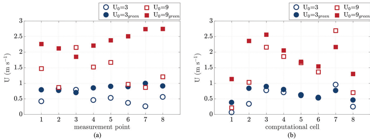
Figure 9. Comparison between the wind speed from the baseline and the green scenario: (a) measured in the wind tunnel and (b) simulated with the CFD model. These results are obtained from the numerical and physical simulations with an inflow wind blowing from North.
