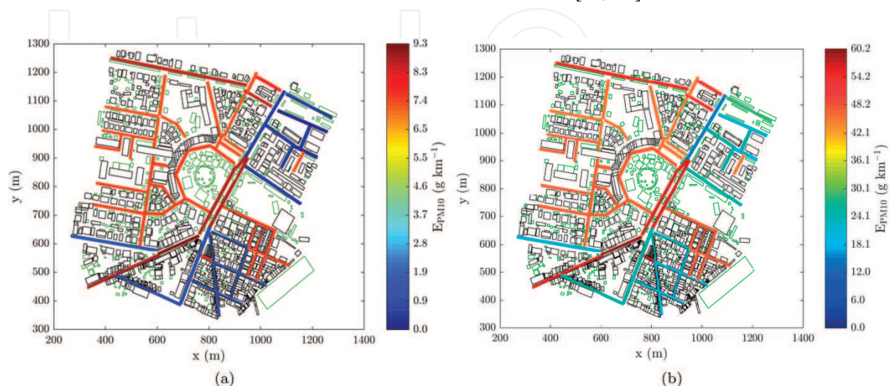
Figure 4. Hourly averaged PM 10 emission rates calculated for each road segment at (a) 4 am and (b) 8 am.
