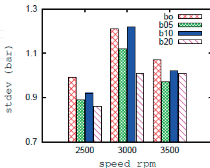
Figure 6. Standard deviation of indicated pressure [21].
