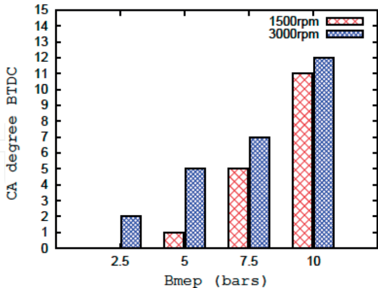
Figure 1. Effect of test fuels on injection timing.
