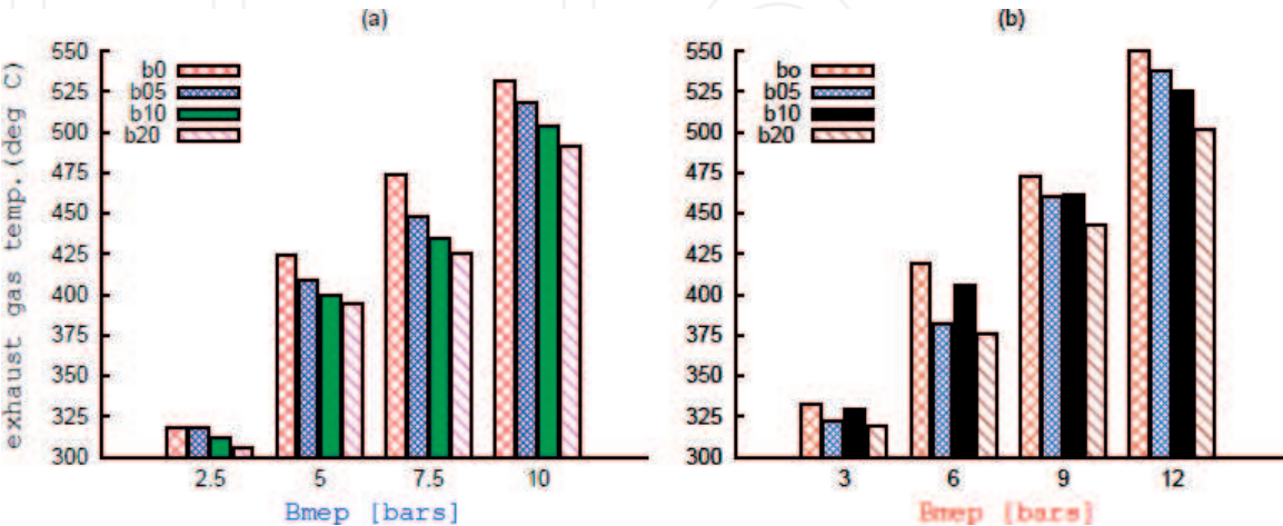
Figure 4. EGT vs. BMEP (a) at 1500 rpm and (b) at 3000 rpm [21].
