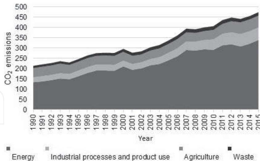
Figure 2. Greenhouse gas emissions according to the sectors in Turkey [34].
