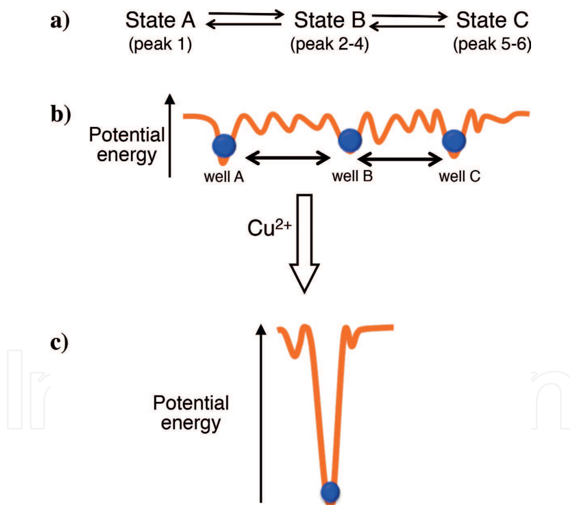
Figure 17. Consideration about conversion of unstable forms to a stable form of CL. (a) State A (corresponding to peak 1 in Figure 10 ), State B (corresponding to peaks 2, 3, and 4 in Figure 10 ), and State C (corresponding to peaks 5 and 6 in Figure 10 ) may stay in a chemical equilibrium. (b) Assumed situation in potential energy for the case without \text{Cu}^{2+} : each potential energy level for the case without \text{Cu}^{2+} may be comparable in wells of A, B, and C. The walls among the potential energy wells are not high. (c) Assumed situation of potential energy for the case with \text{Cu}^{2+} : when \text{Cu}^{2+} is incorporated, a deep potential level can be generated, and all molecules showing a different heterogeneity may drop into the well and exist as a stable form.
