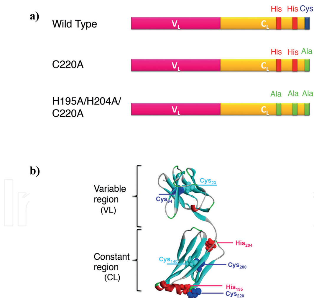
Figure 18. C51 mutants and locations of His and Cys residues. There are no histidine residues in the variable region of the C51 light chain. (a) Location of Cys220, His195 and His204 in wild type. The mutated positions, C220A and H195A/H204A/C220A, are also indicated with green colored character. (b) Three-dimensional structure of the C51 light chain. Light blue is sheet structure and red is helix structure.
