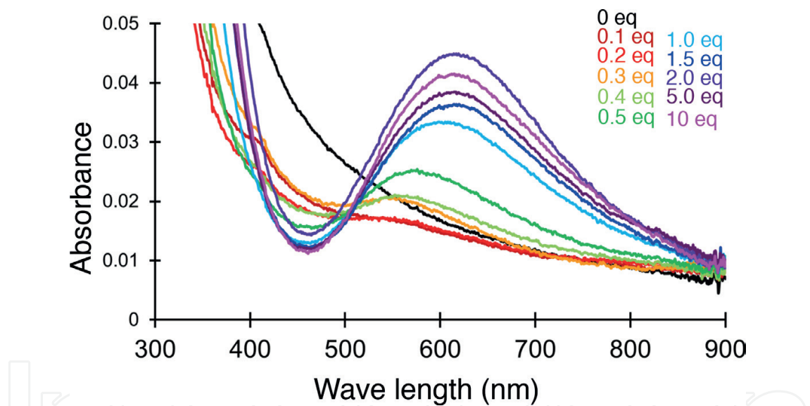
Figure 13. Spectrum changes with the concentration of added \text{Cu}^{2+} . Along with an increase of the concentration of added \text{Cu}^{2+} , the absorbance at around 580 nm became larger.
