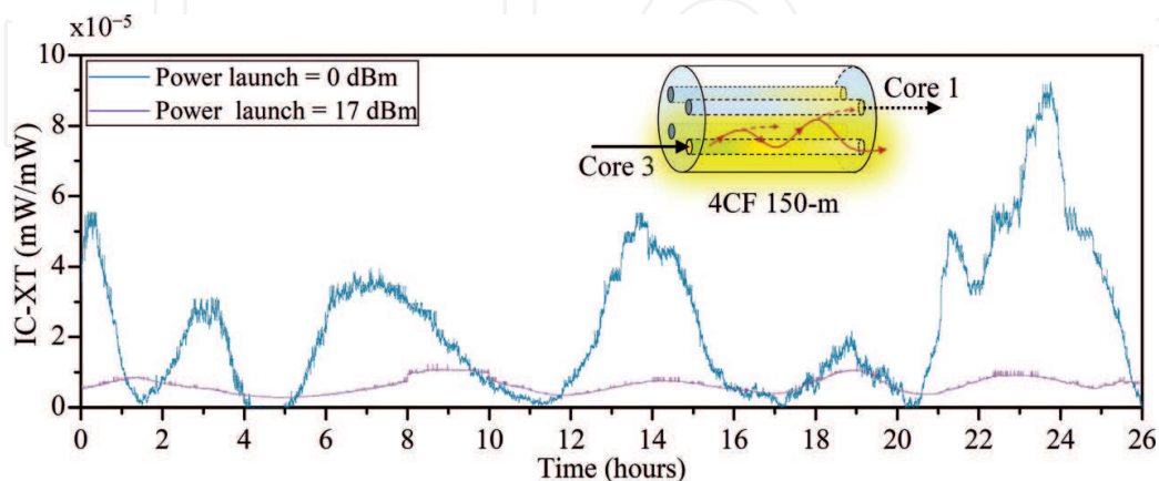
Figure 2. Measured temporal profile of the linear and nonlinear IC-XT between adjacent cores in a homogeneous 4-core MCF (results based on [49]).
