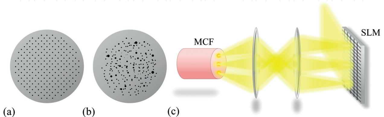
Figure 11. MCFs and adaptive optics for medical imaging. (a) MCF with low IC-XT and periodically arranged cores [113], (b) disorder MCF based on transverse Anderson localization, and (c) wavefront shaping with a single spatial light modulator (SLM) for a MCF based lensless endoscope. Results based on [22, 114].
