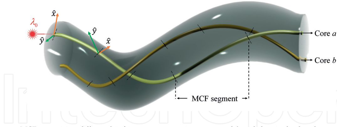
Figure 3. MCF comprising different birefringent segments in cores a and b with longitudinal and temporal varying fluctuations in the first-order electrical permittivity tensor.
