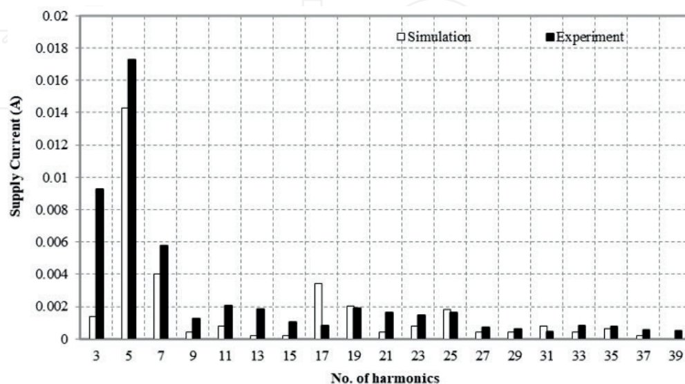
Figure 6. Harmonic spectrum before the compensation.
