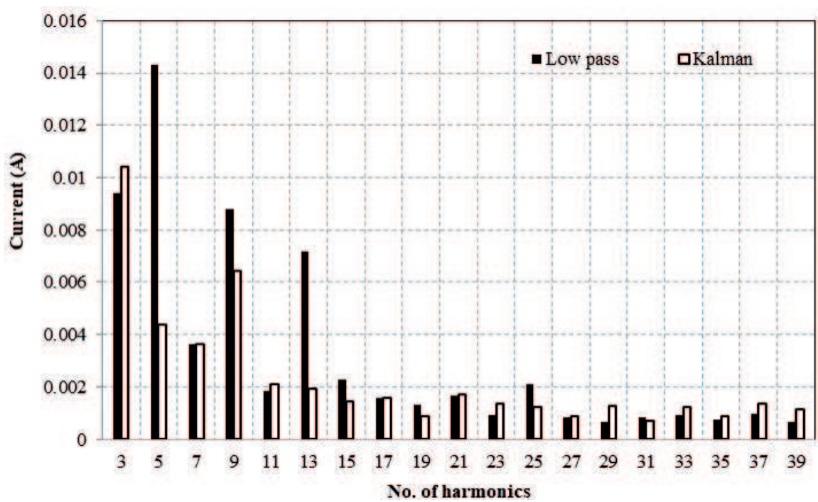
Figure 13. Harmonics spectrum.
