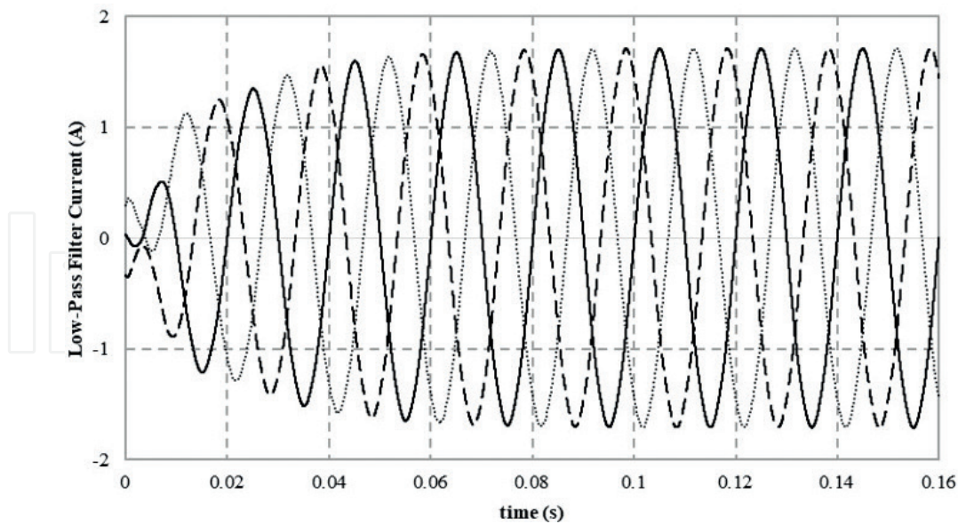
Figure 9. Experimental Butterworth low-pass filter.
