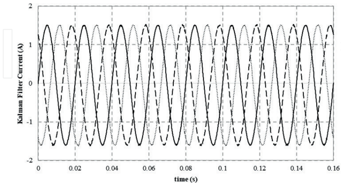
Figure 10. Experiment of Kalman filter.
