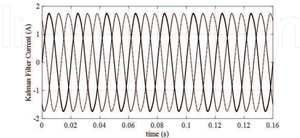
Figure 8. Simulation of Kalman filter.
